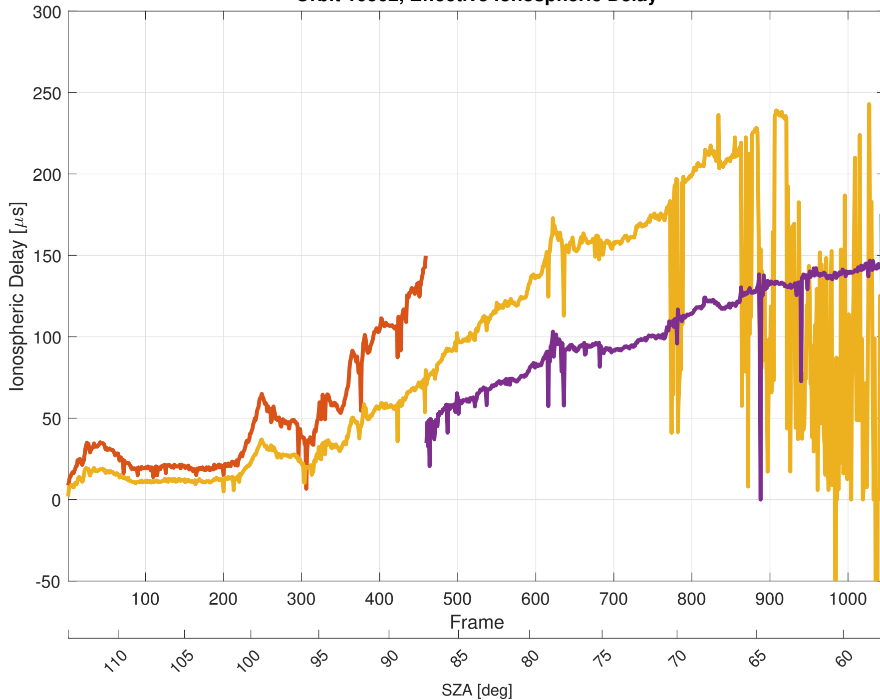
Orbit 10562, Effective Ionospheric Delay
