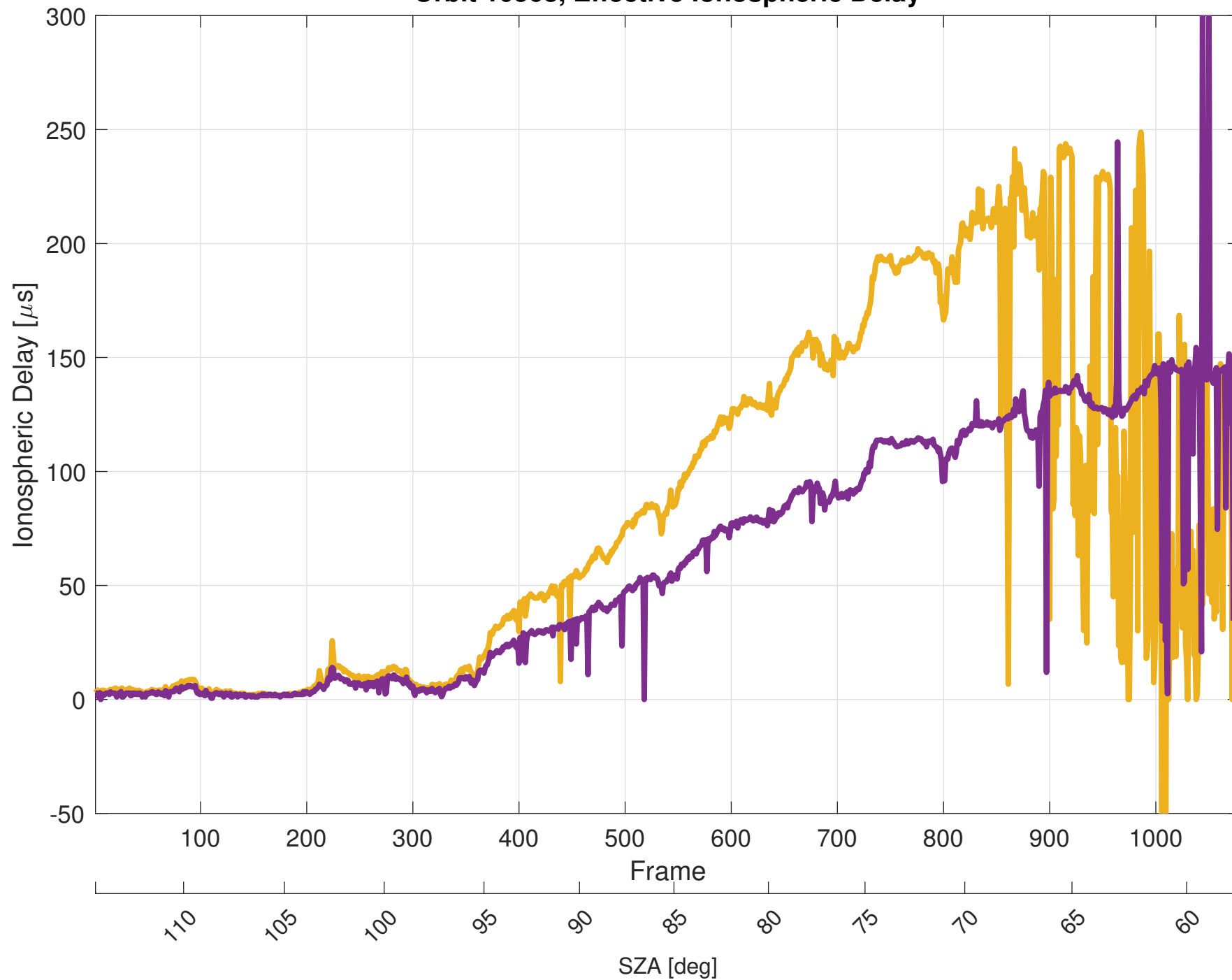
Orbit 10568, Effective Ionospheric Delay
