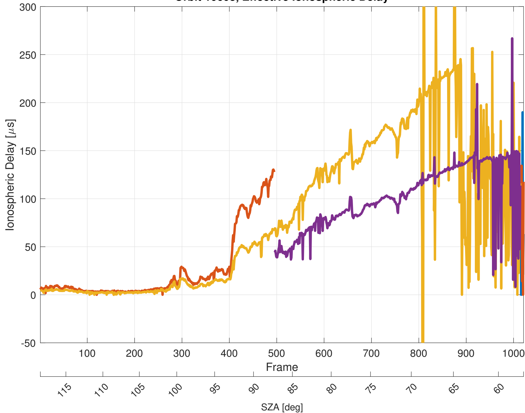
Orbit 10603, Effective Ionospheric Delay
