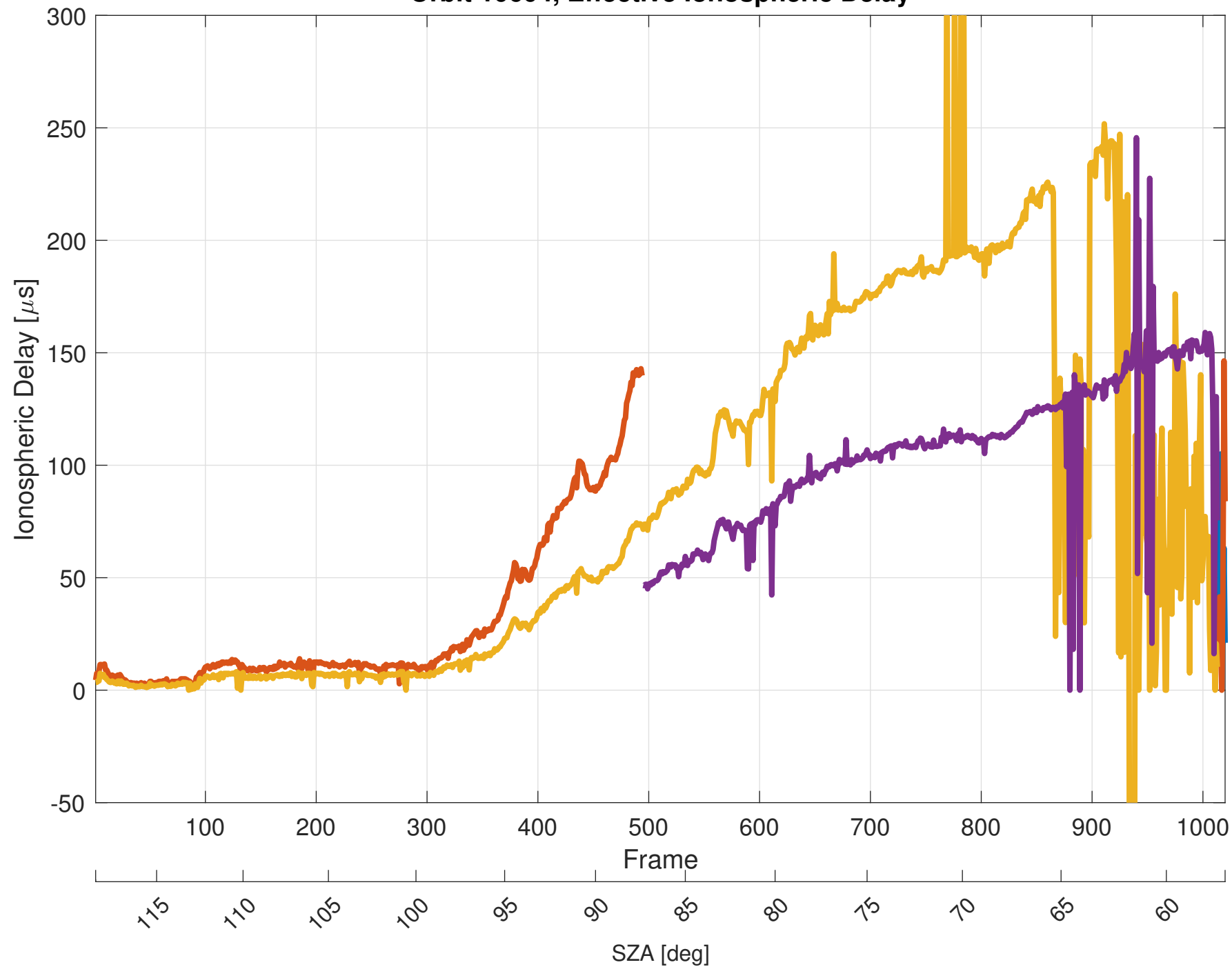
Orbit 10604, Effective Ionospheric Delay
