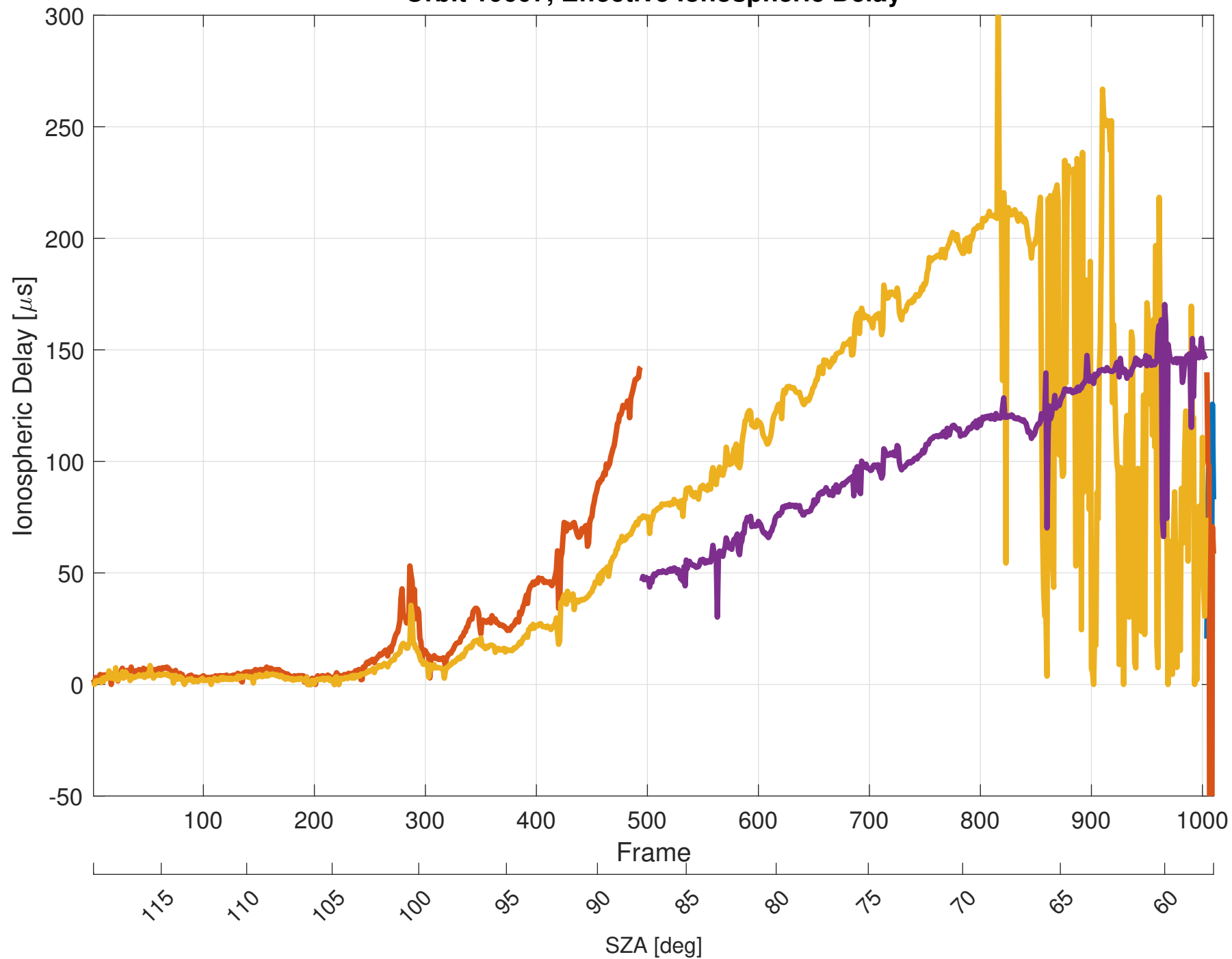
Orbit 10607, Effective Ionospheric Delay
