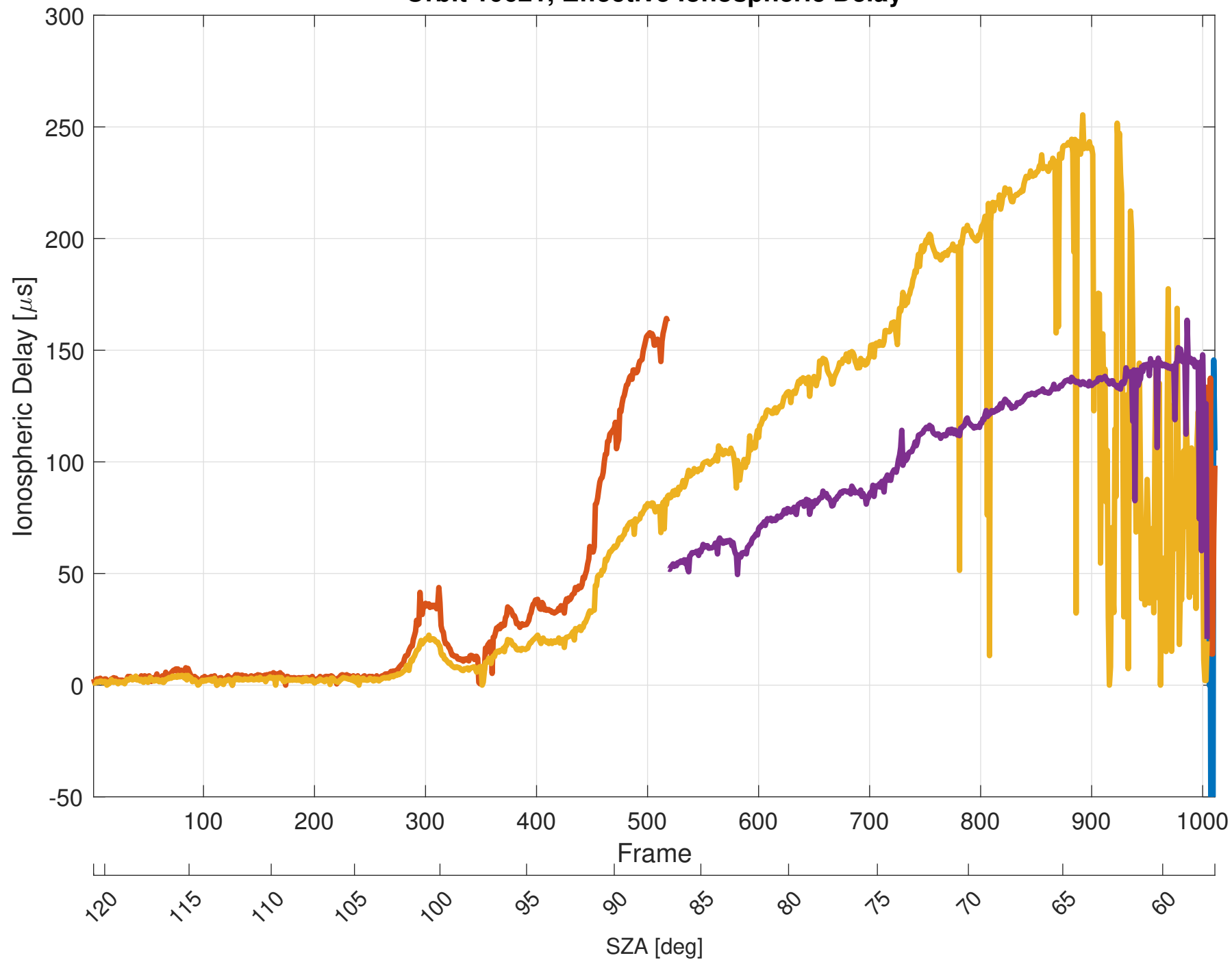
Orbit 10621, Effective Ionospheric Delay
