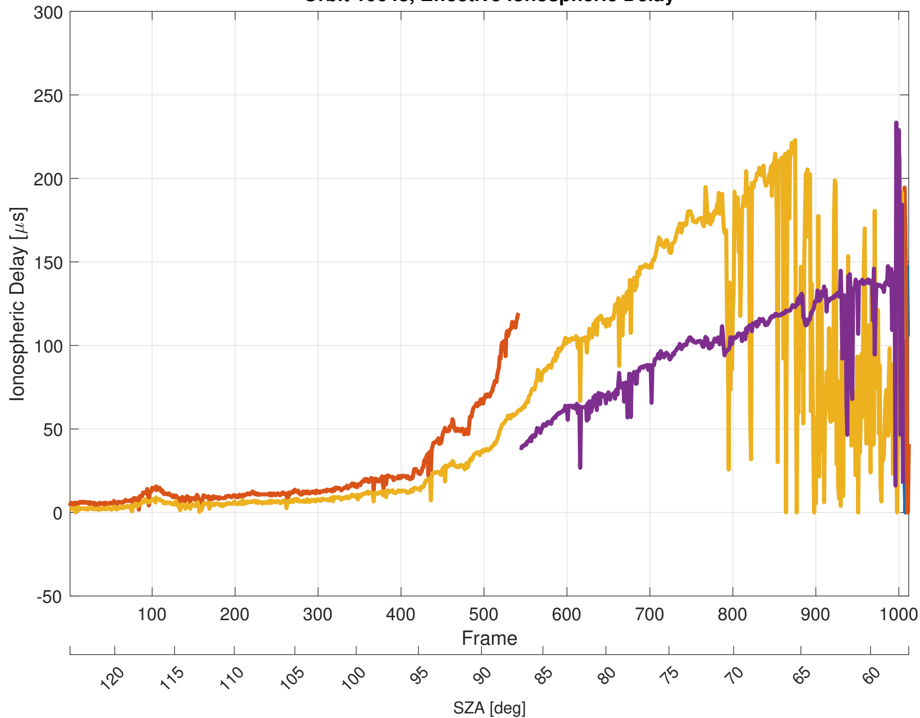
Orbit 10643, Effective Ionospheric Delay
