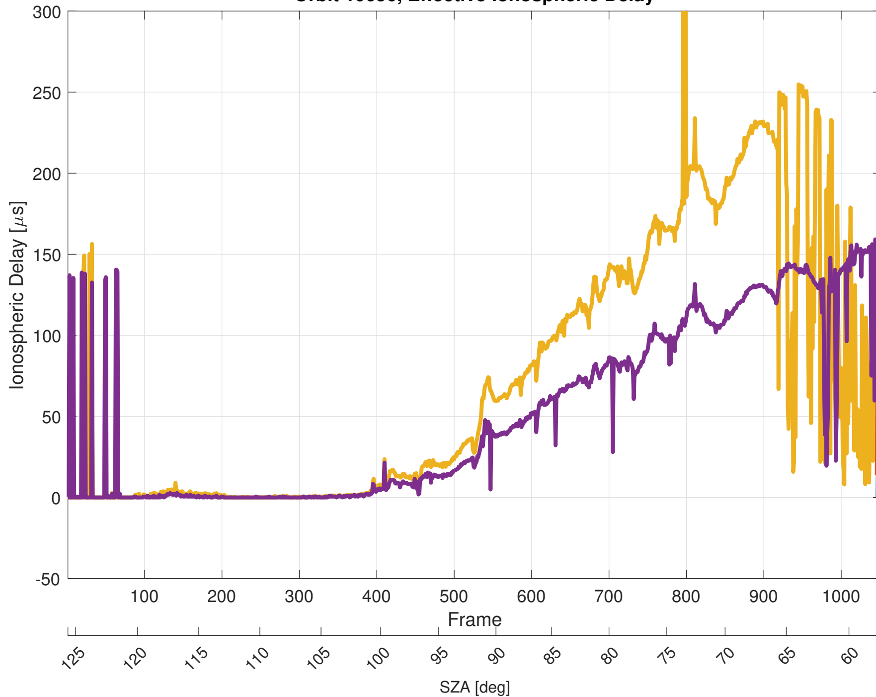
Orbit 10656, Effective Ionospheric Delay
