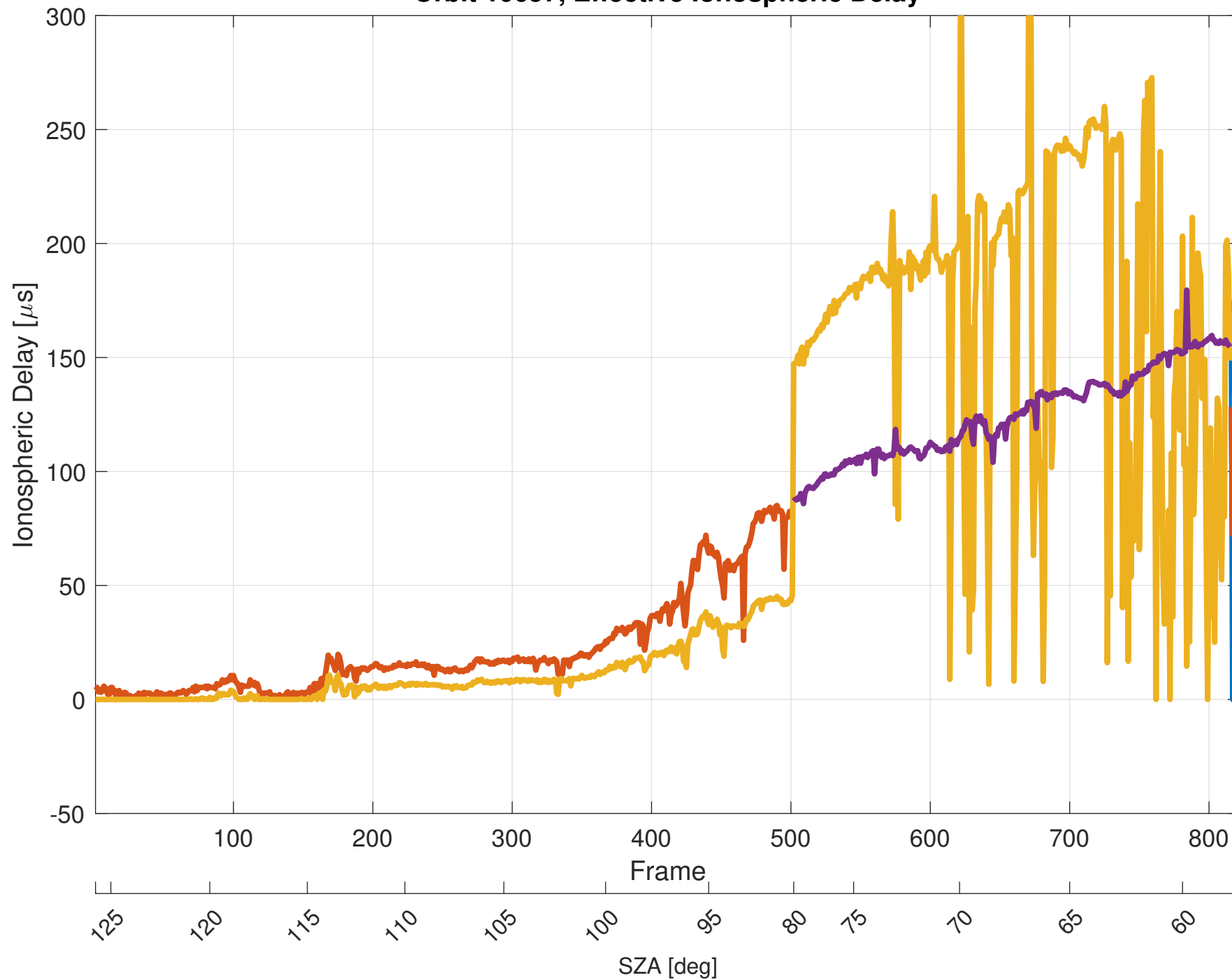
Orbit 10657, Effective Ionospheric Delay
