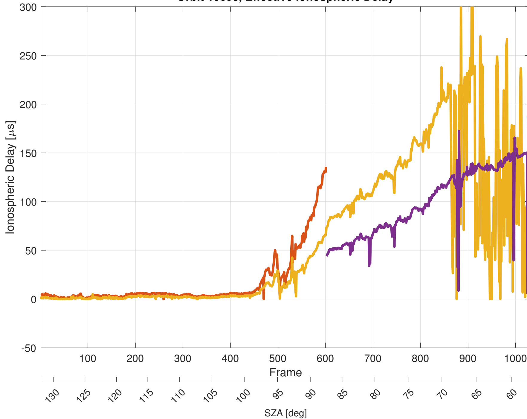
Orbit 10698, Effective Ionospheric Delay
