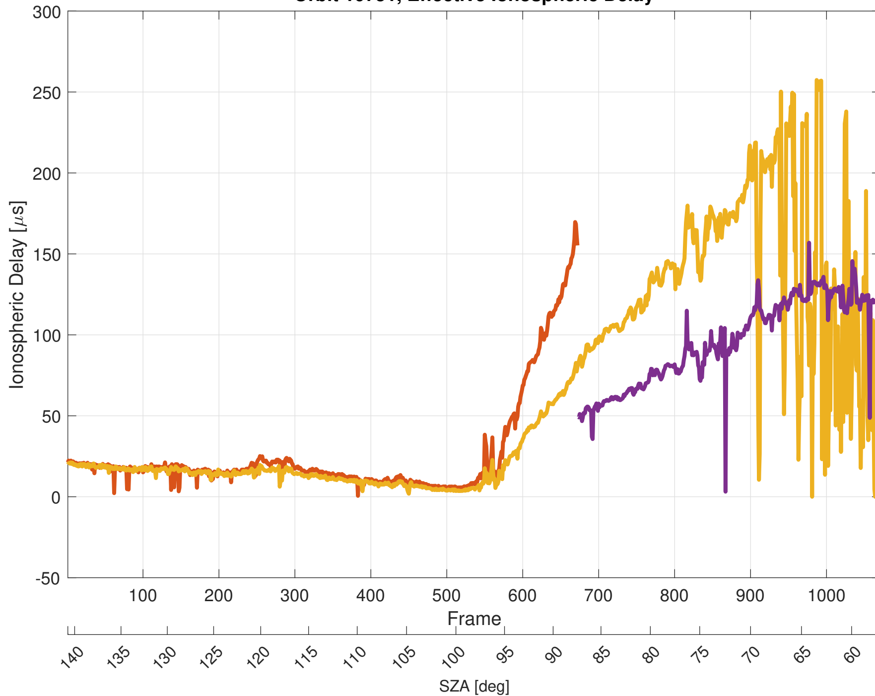
Orbit 10751, Effective Ionospheric Delay
