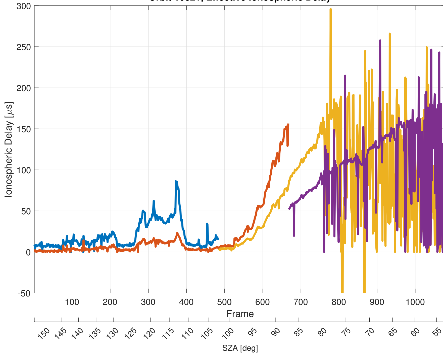
Orbit 10821, Effective Ionospheric Delay
