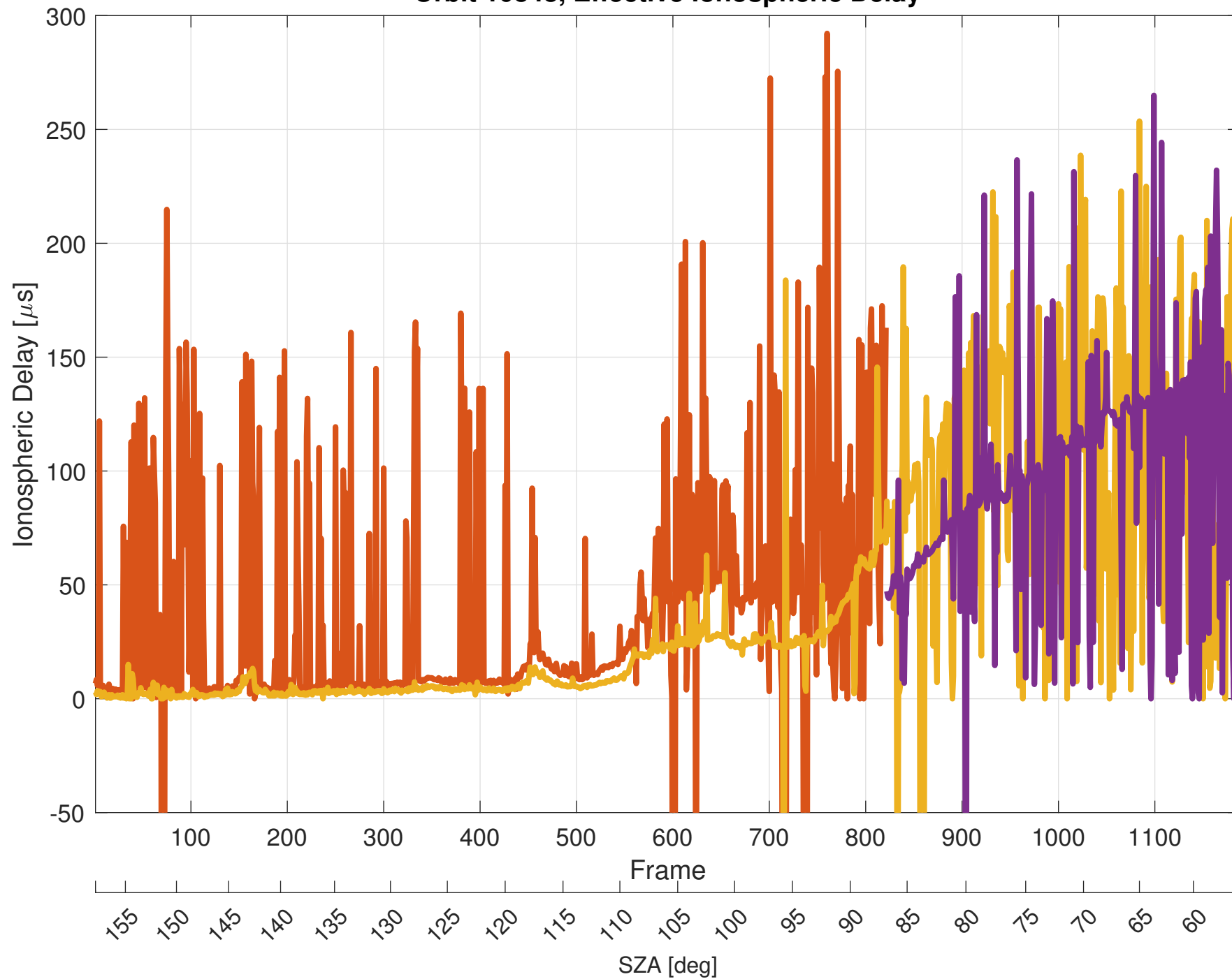
Orbit 10848, Effective Ionospheric Delay
