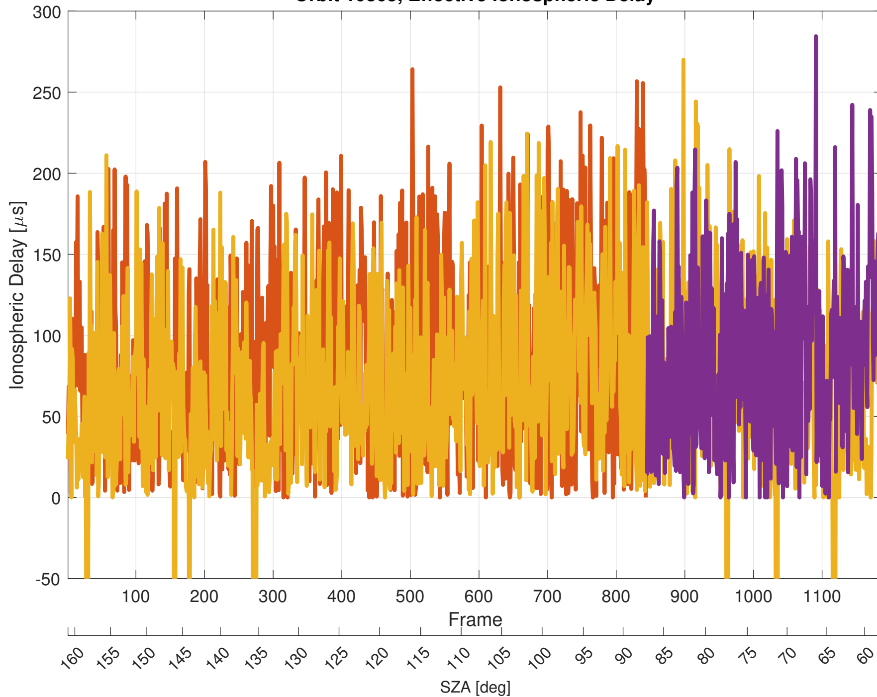
Orbit 10865, Effective Ionospheric Delay
