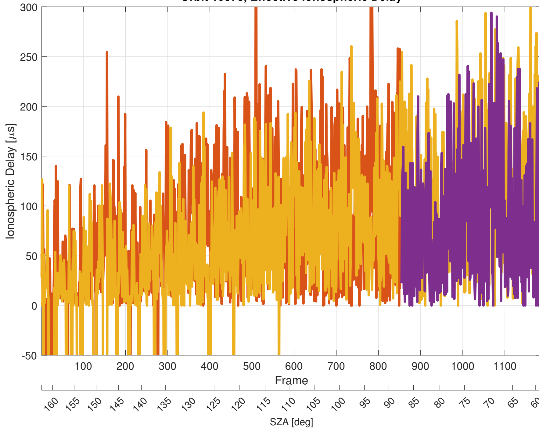
Orbit 10873, Effective Ionospheric Delay
