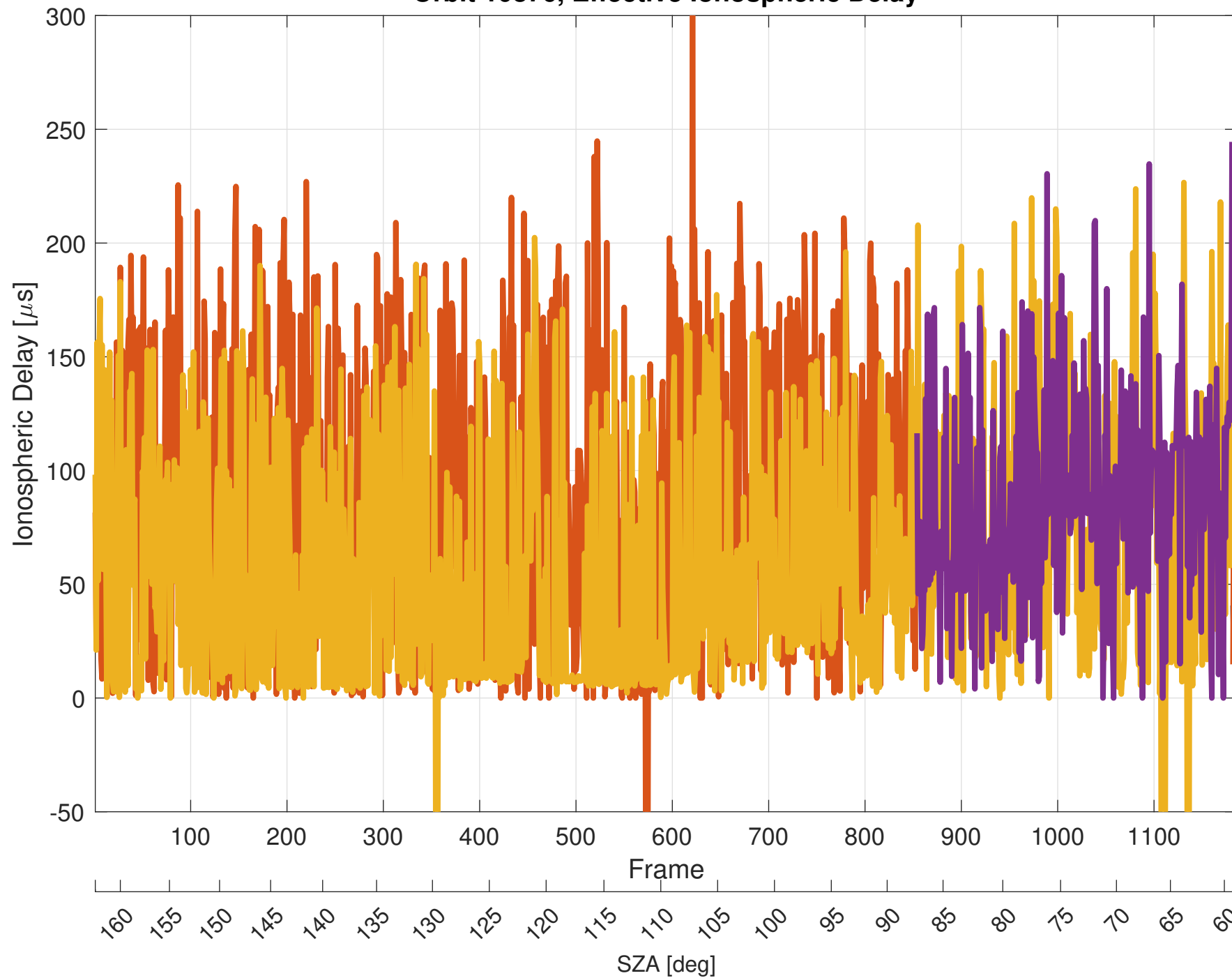
Orbit 10876, Effective Ionospheric Delay
