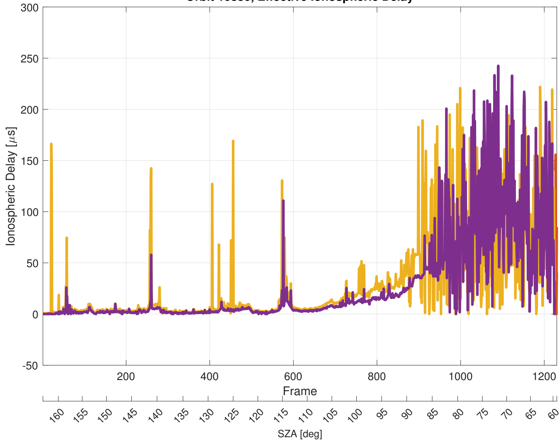
Orbit 10880, Effective Ionospheric Delay
