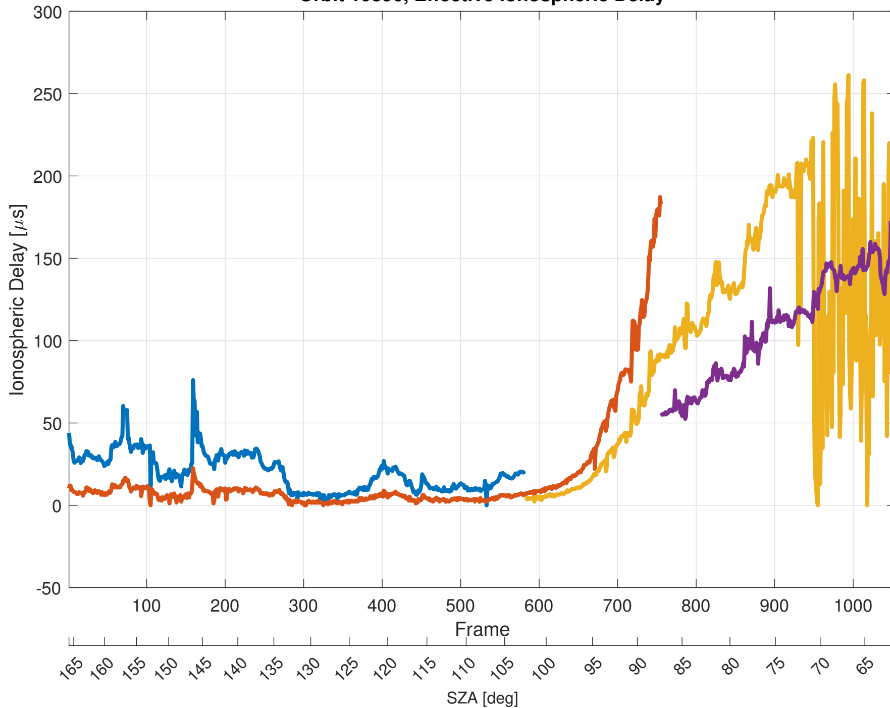
Orbit 10896, Effective Ionospheric Delay
