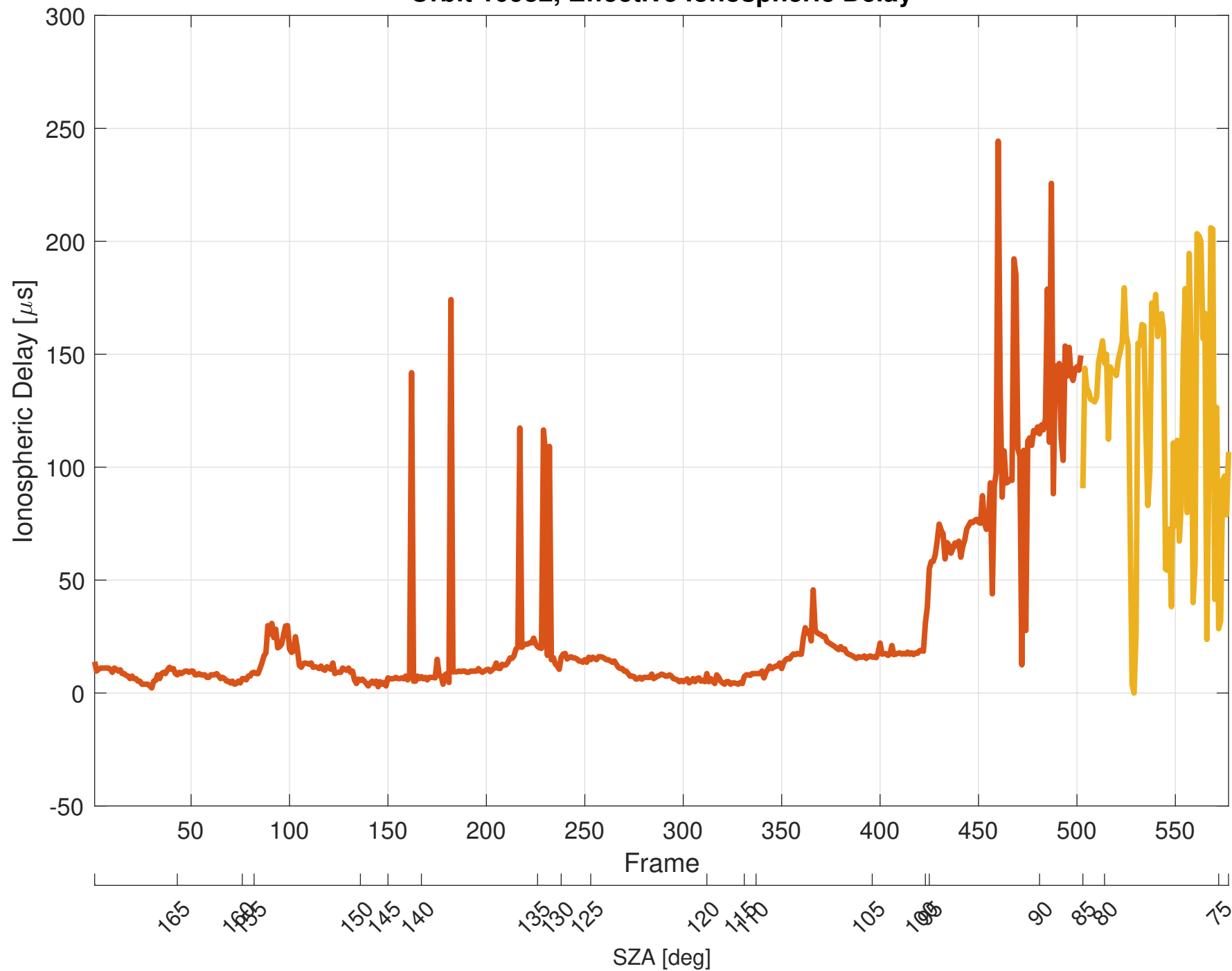
Orbit 10932, Effective Ionospheric Delay
