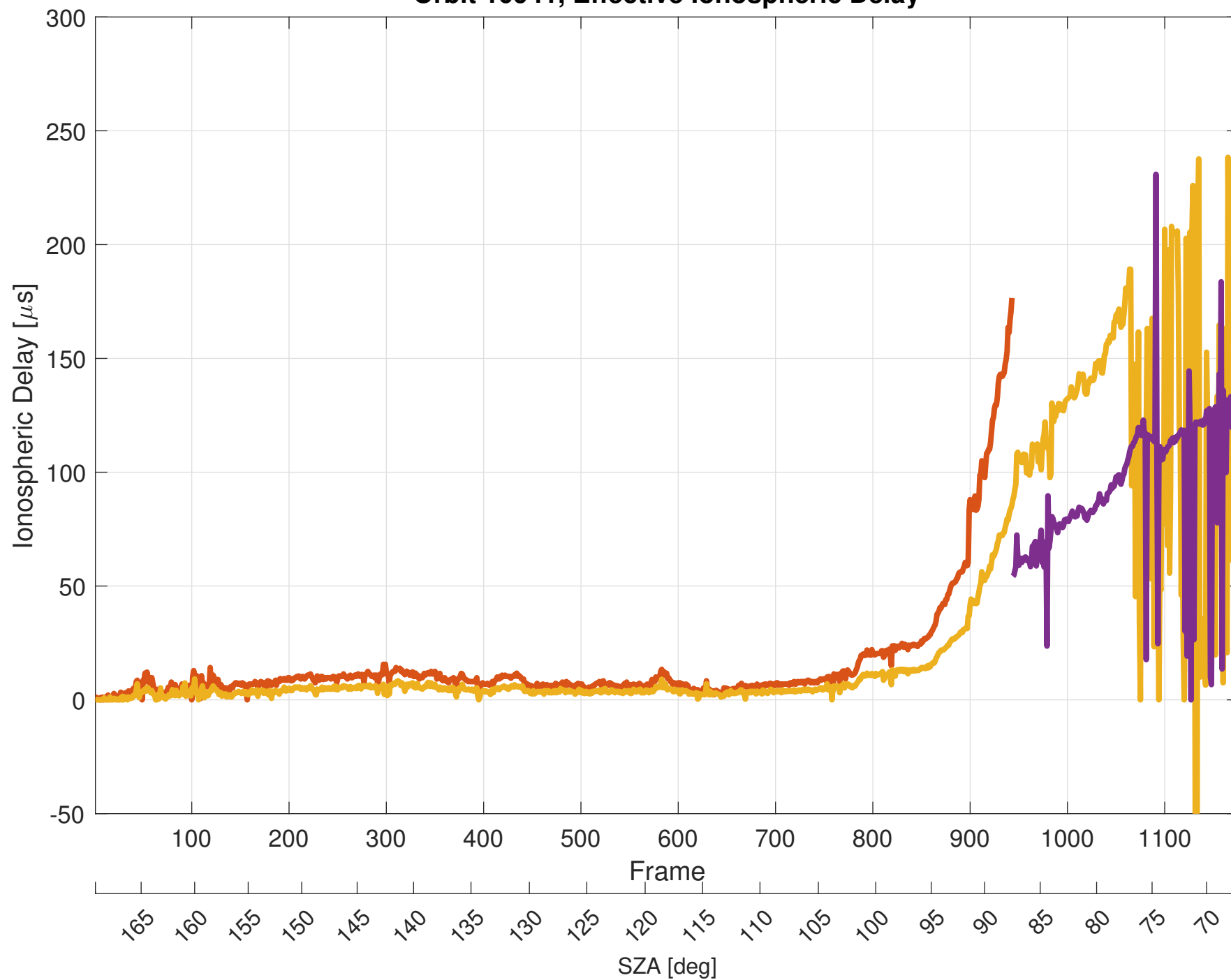
Orbit 10941, Effective Ionospheric Delay
