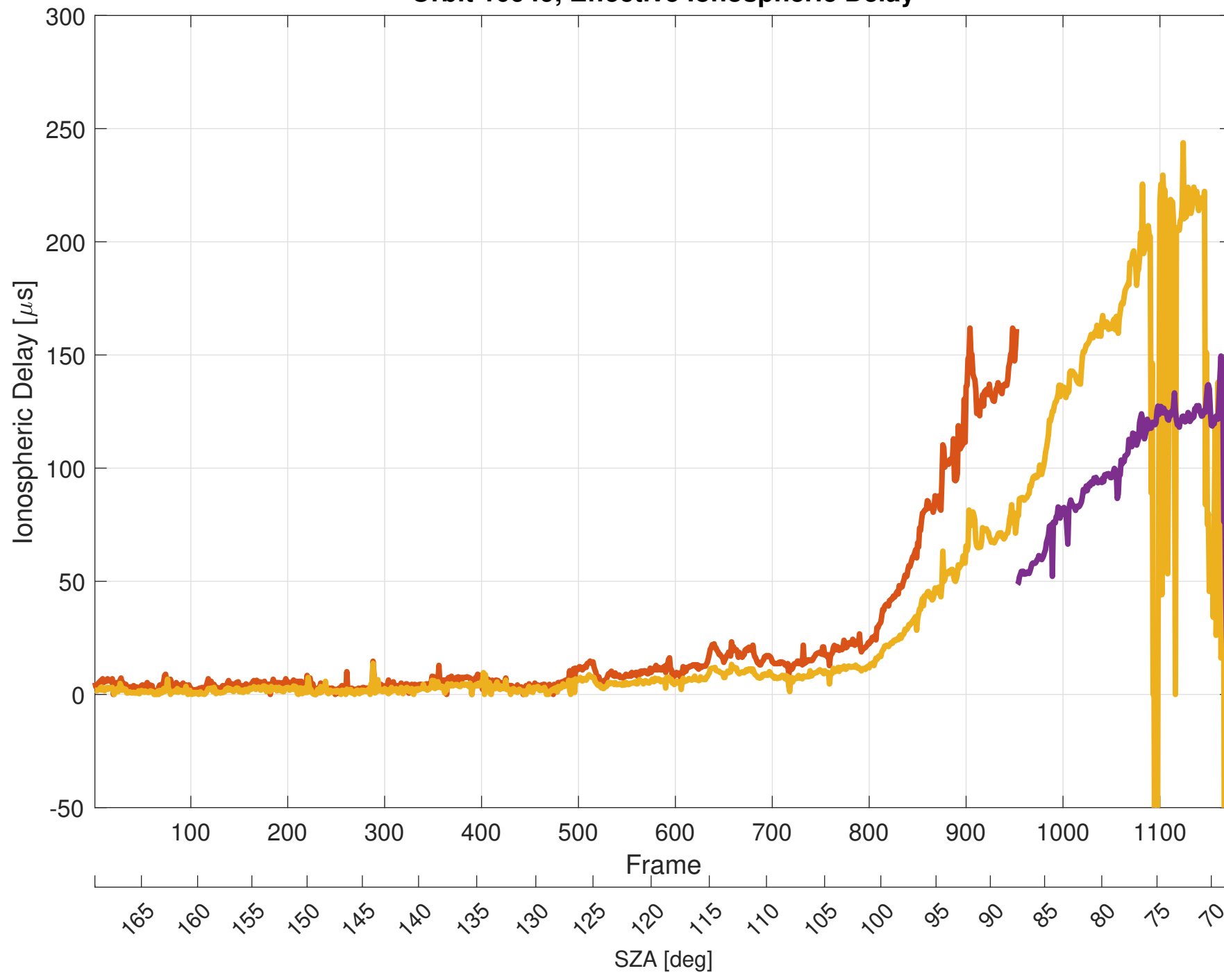
Orbit 10949, Effective Ionospheric Delay
