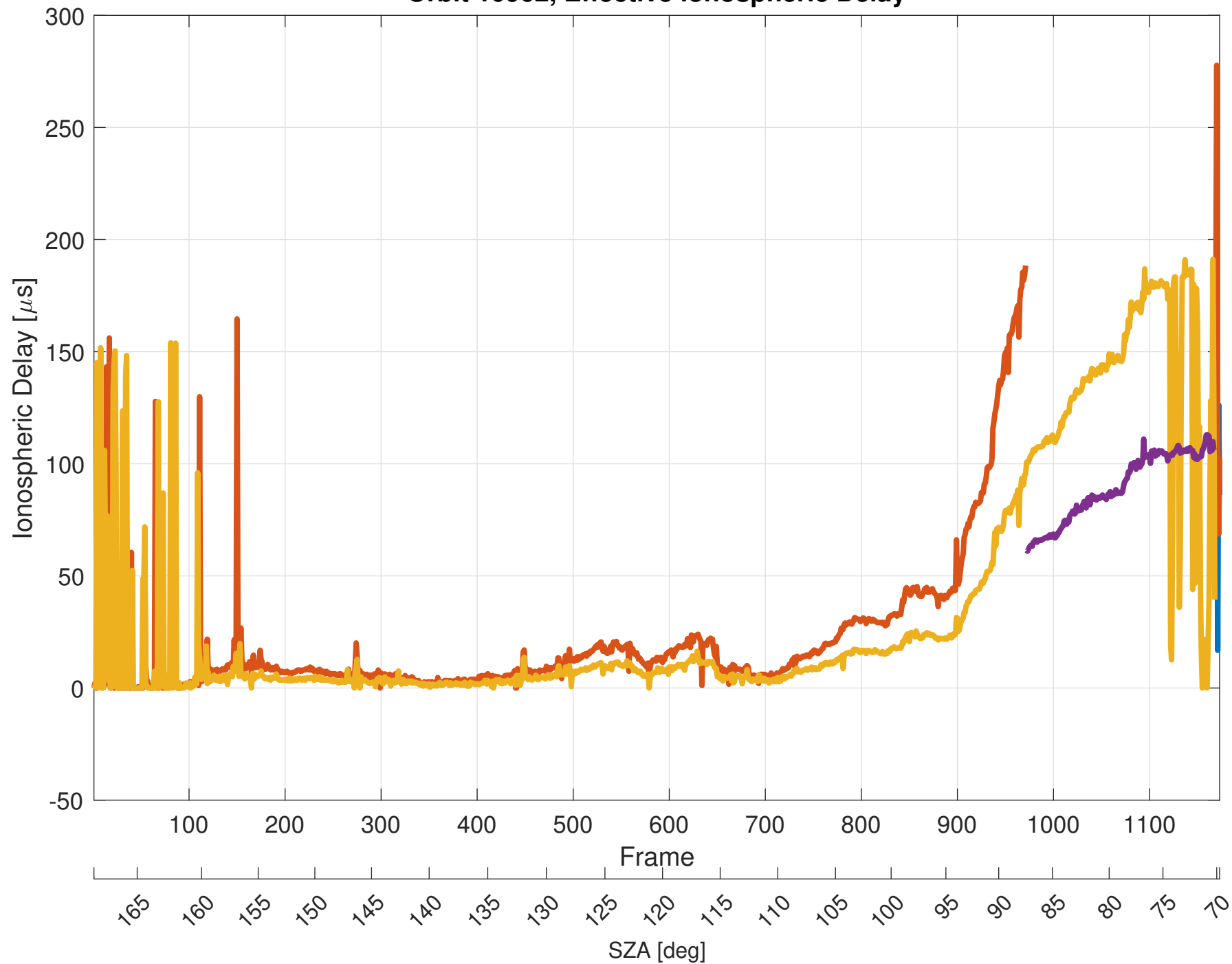
Orbit 10962, Effective Ionospheric Delay
