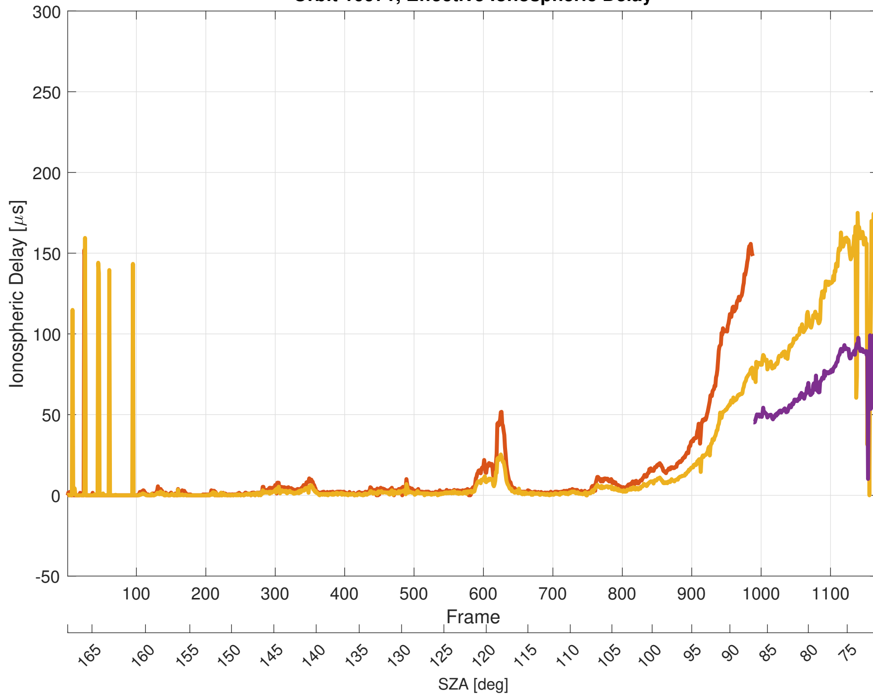
Orbit 10971, Effective Ionospheric Delay
