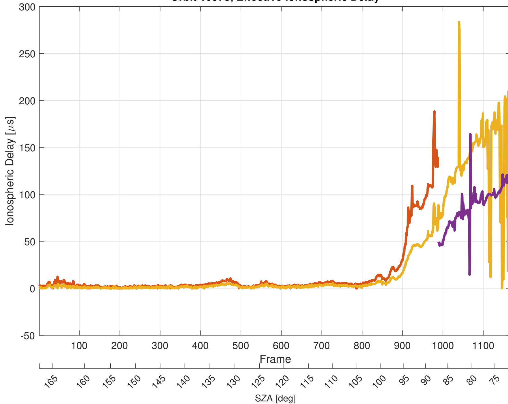
Orbit 10973, Effective Ionospheric Delay
