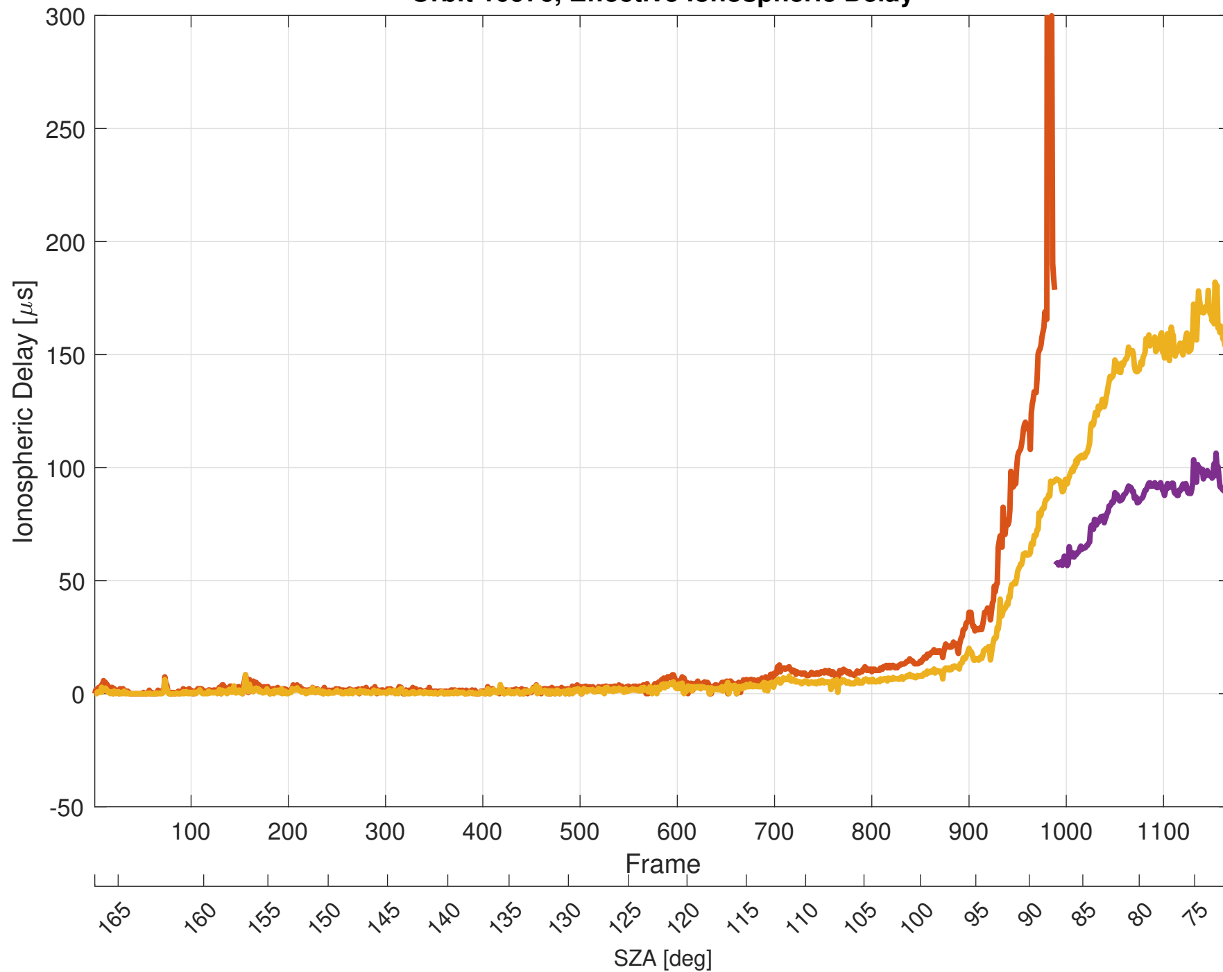
Orbit 10976, Effective Ionospheric Delay
