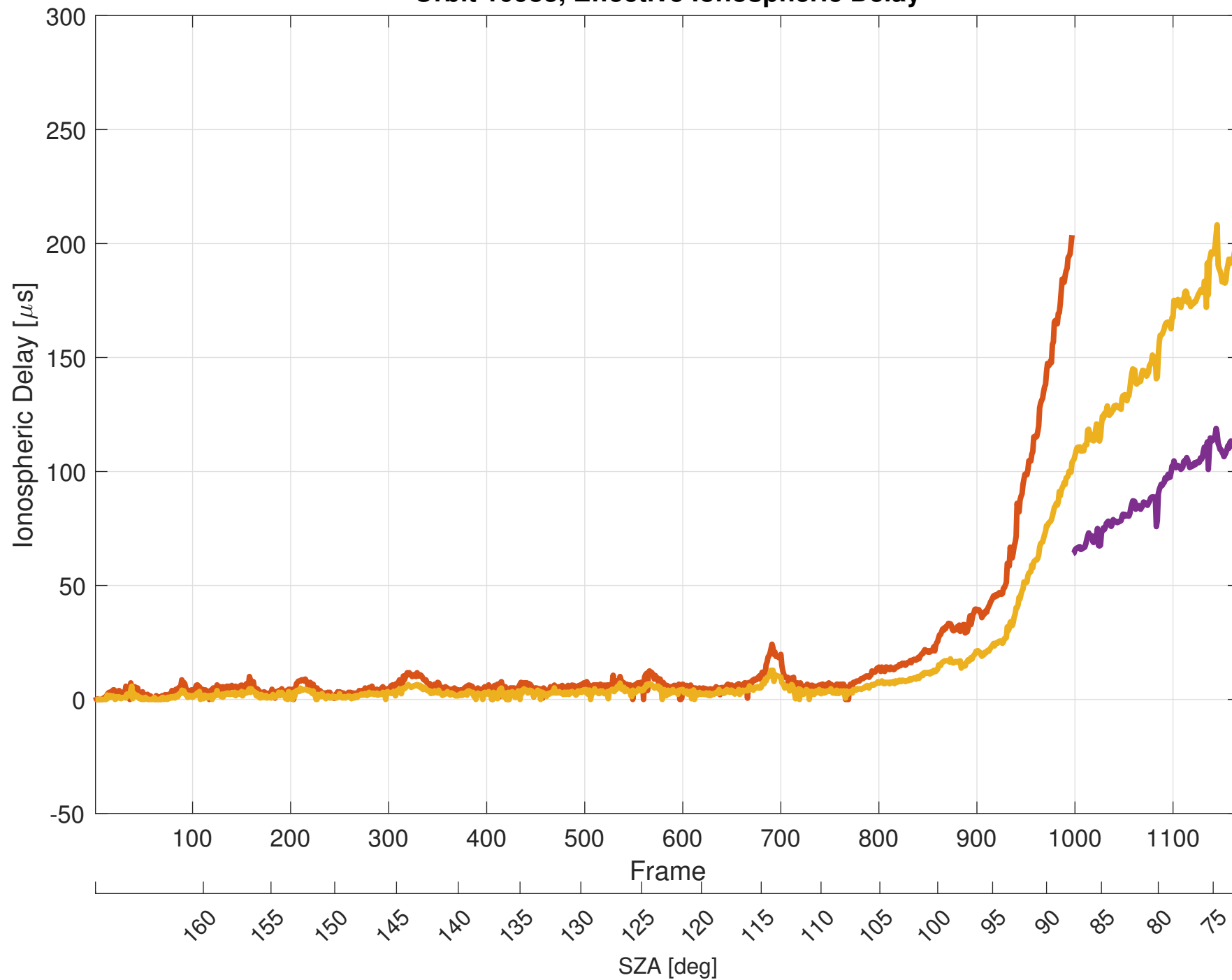
Orbit 10983, Effective Ionospheric Delay
