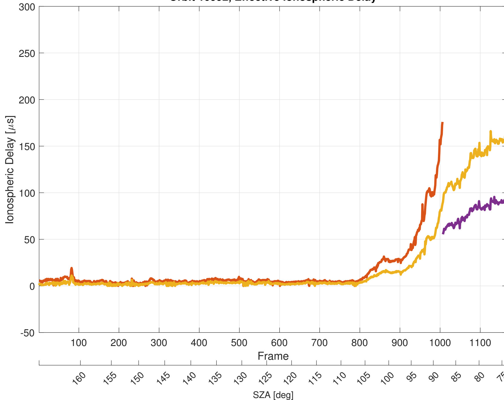
Orbit 10992, Effective Ionospheric Delay
