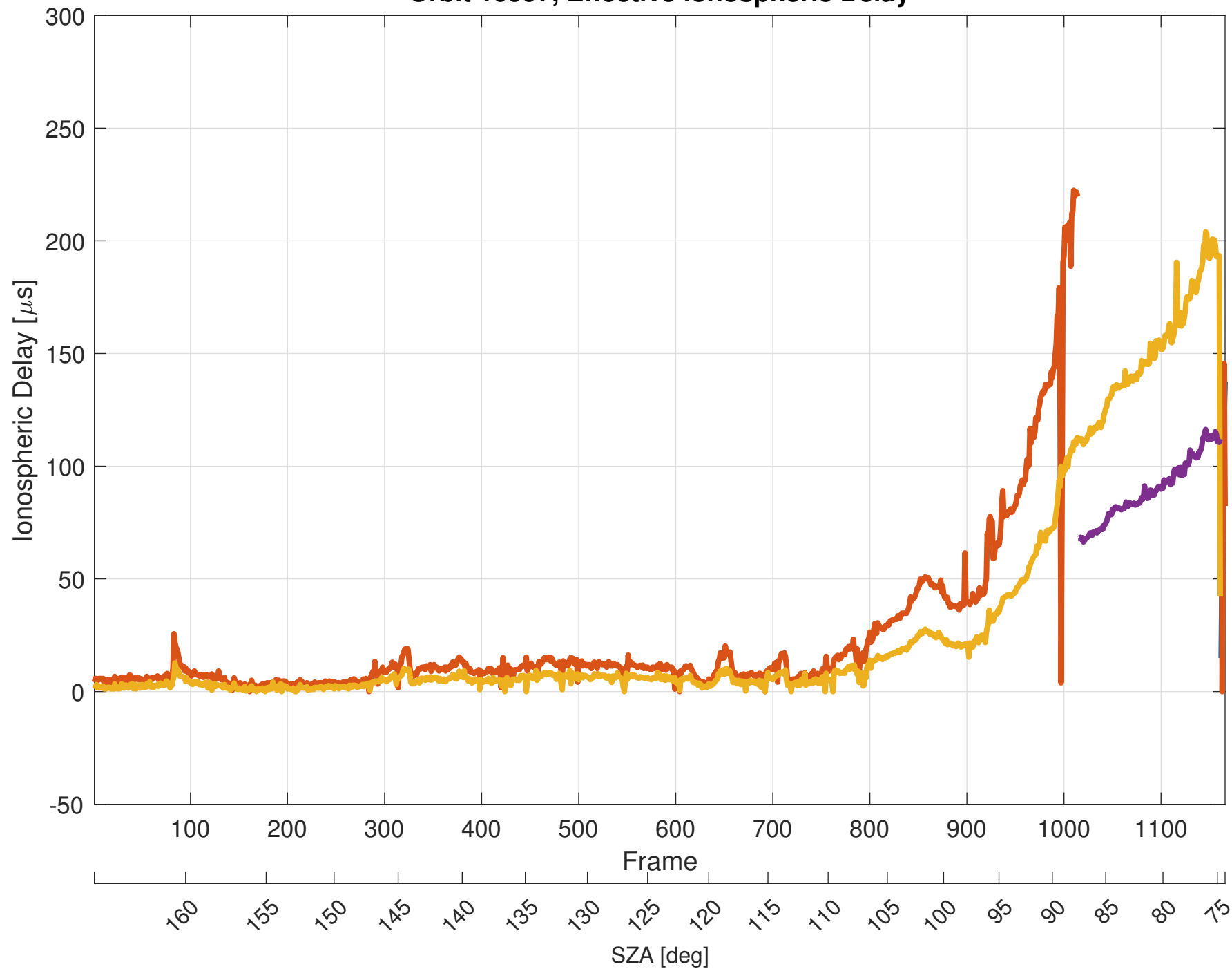
Orbit 10997, Effective Ionospheric Delay
