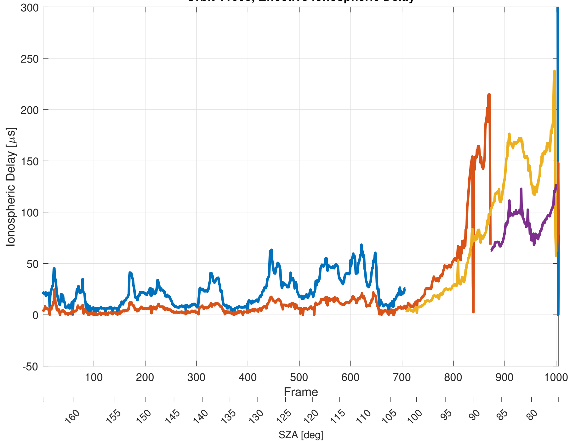
Orbit 11005, Effective Ionospheric Delay
