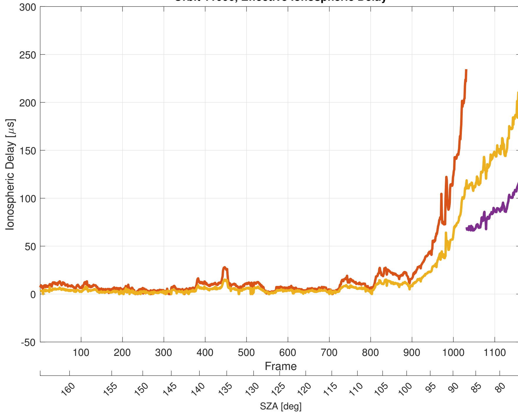
Orbit 11006, Effective Ionospheric Delay
