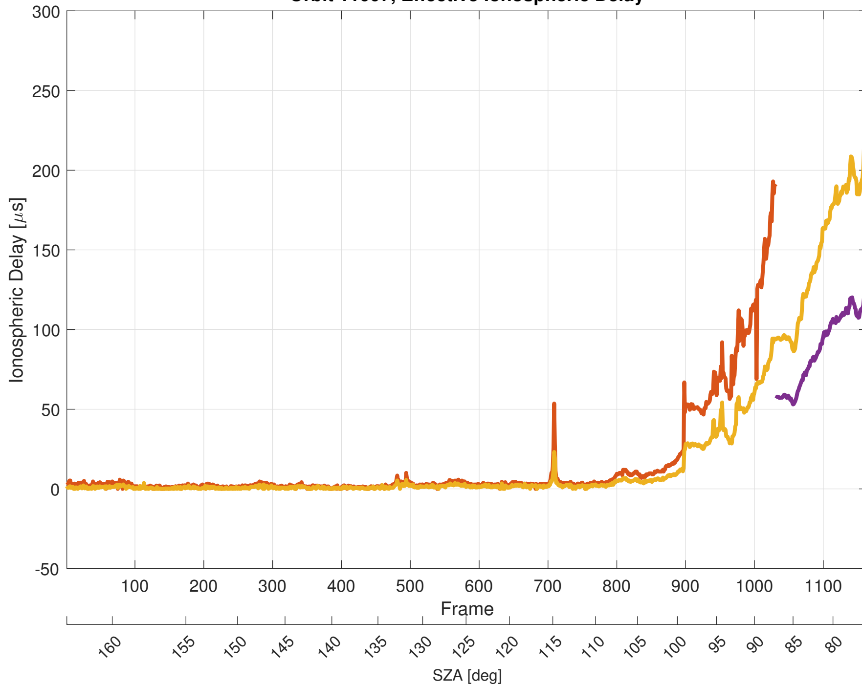
Orbit 11007, Effective Ionospheric Delay
