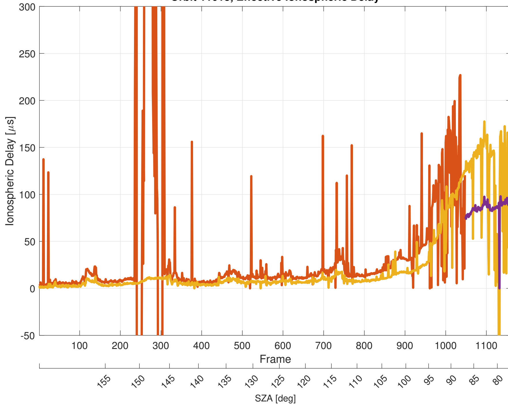
Orbit 11018, Effective Ionospheric Delay
