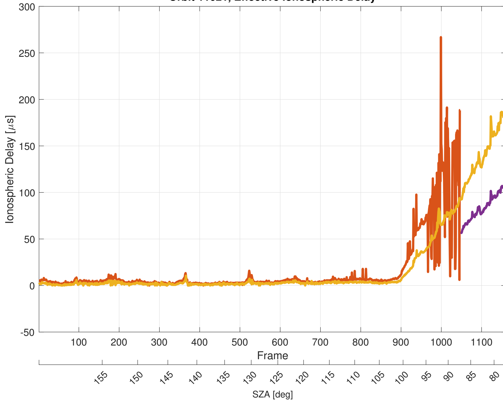
Orbit 11021, Effective Ionospheric Delay
