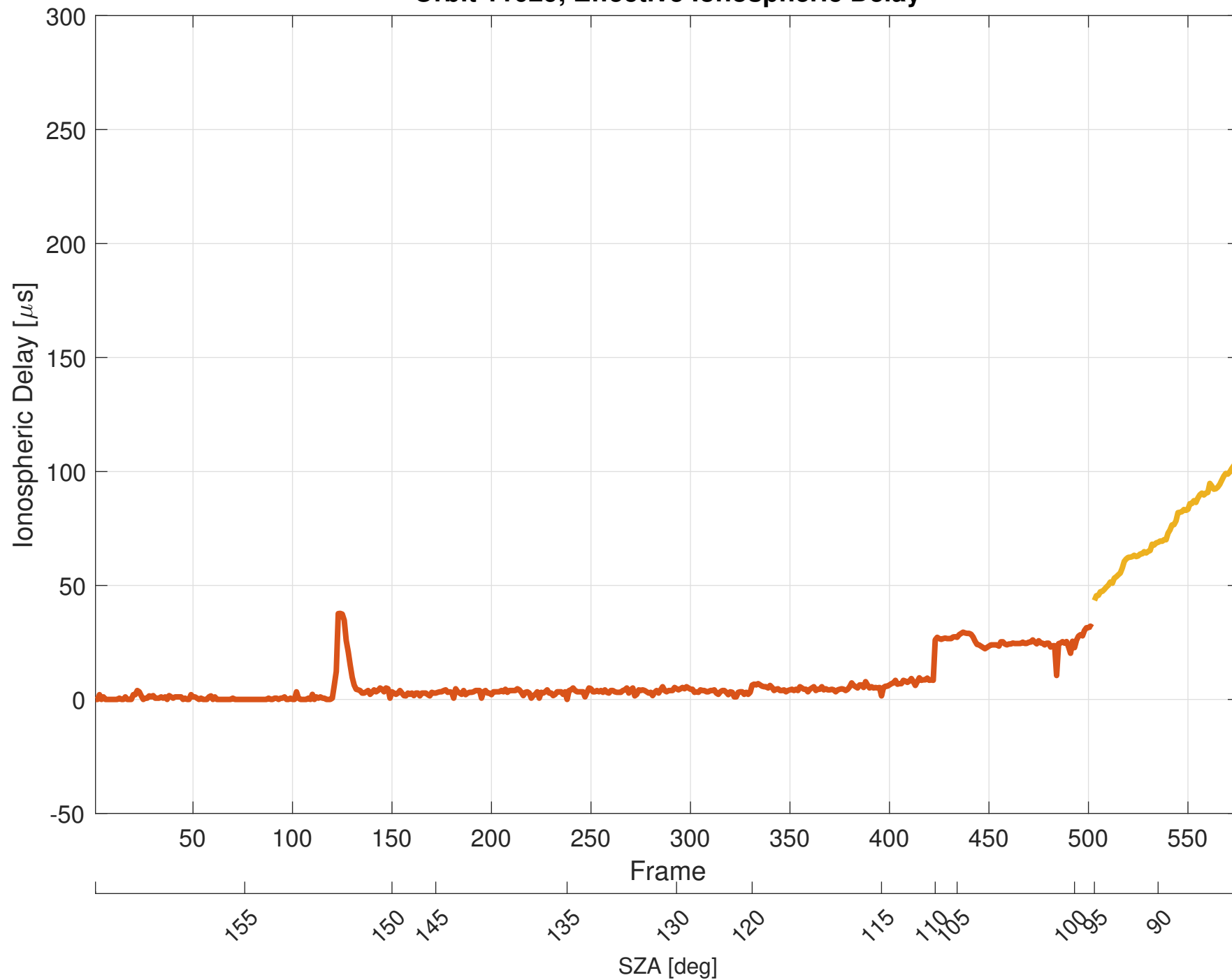
Orbit 11029, Effective Ionospheric Delay
