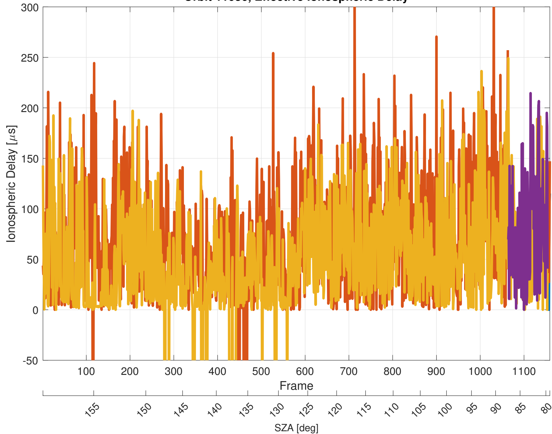
Orbit 11036, Effective Ionospheric Delay
