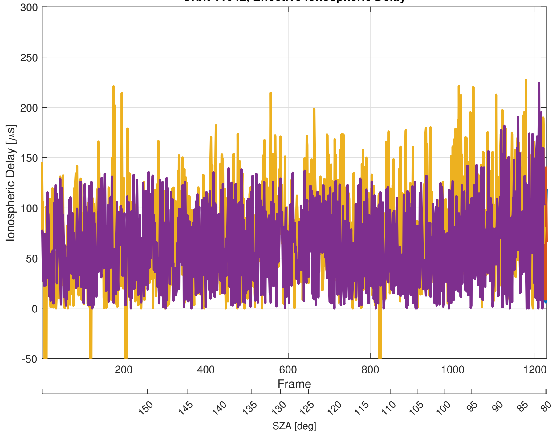
Orbit 11042, Effective Ionospheric Delay
