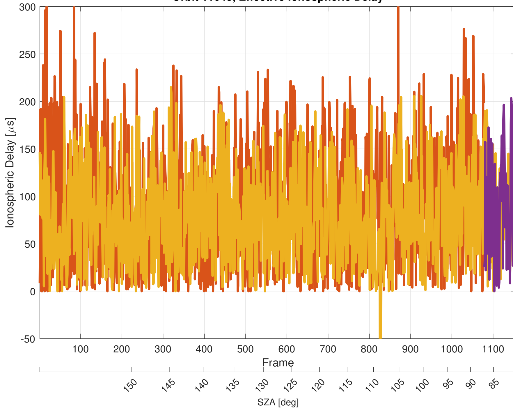
Orbit 11045, Effective Ionospheric Delay
