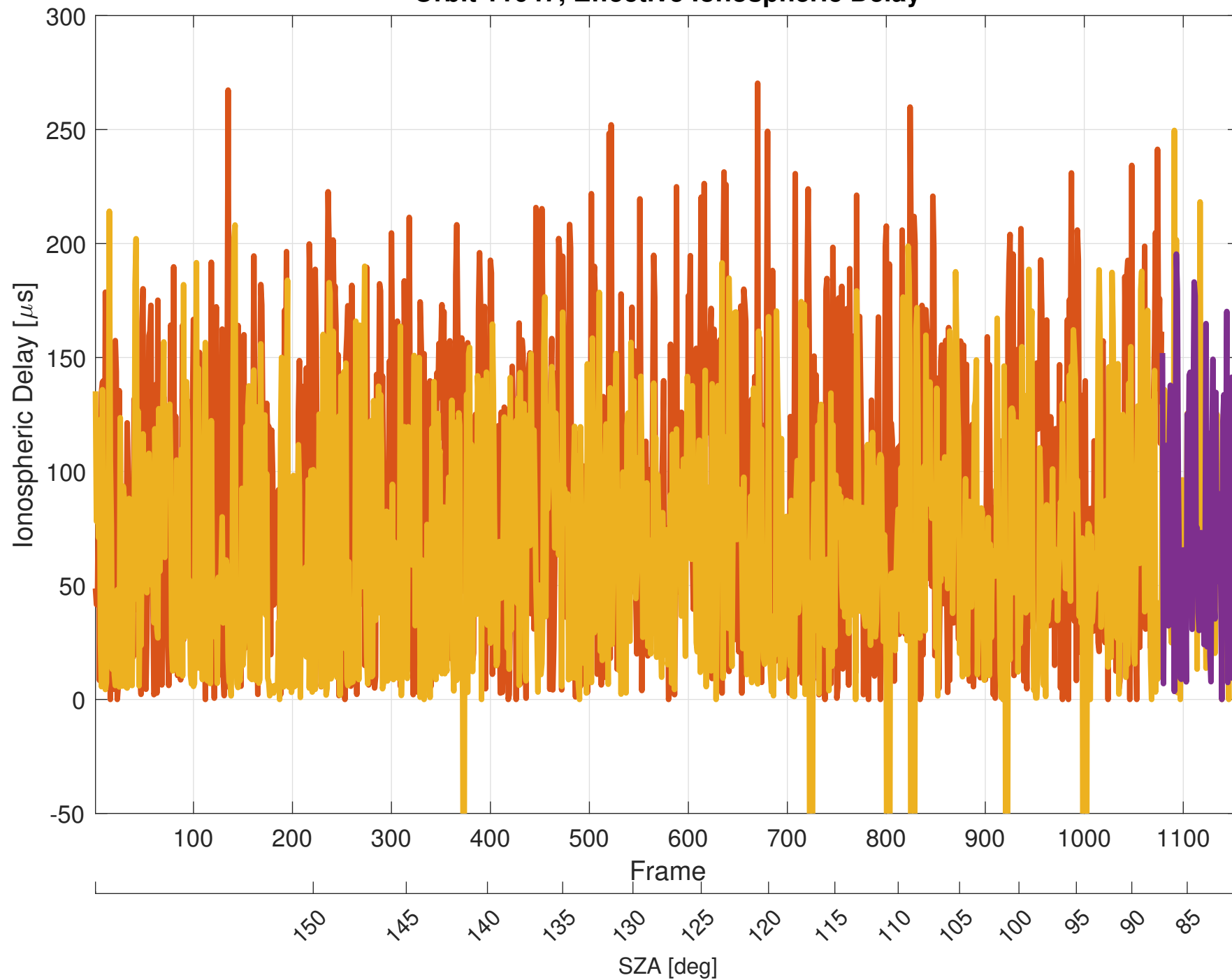
Orbit 11047, Effective Ionospheric Delay
