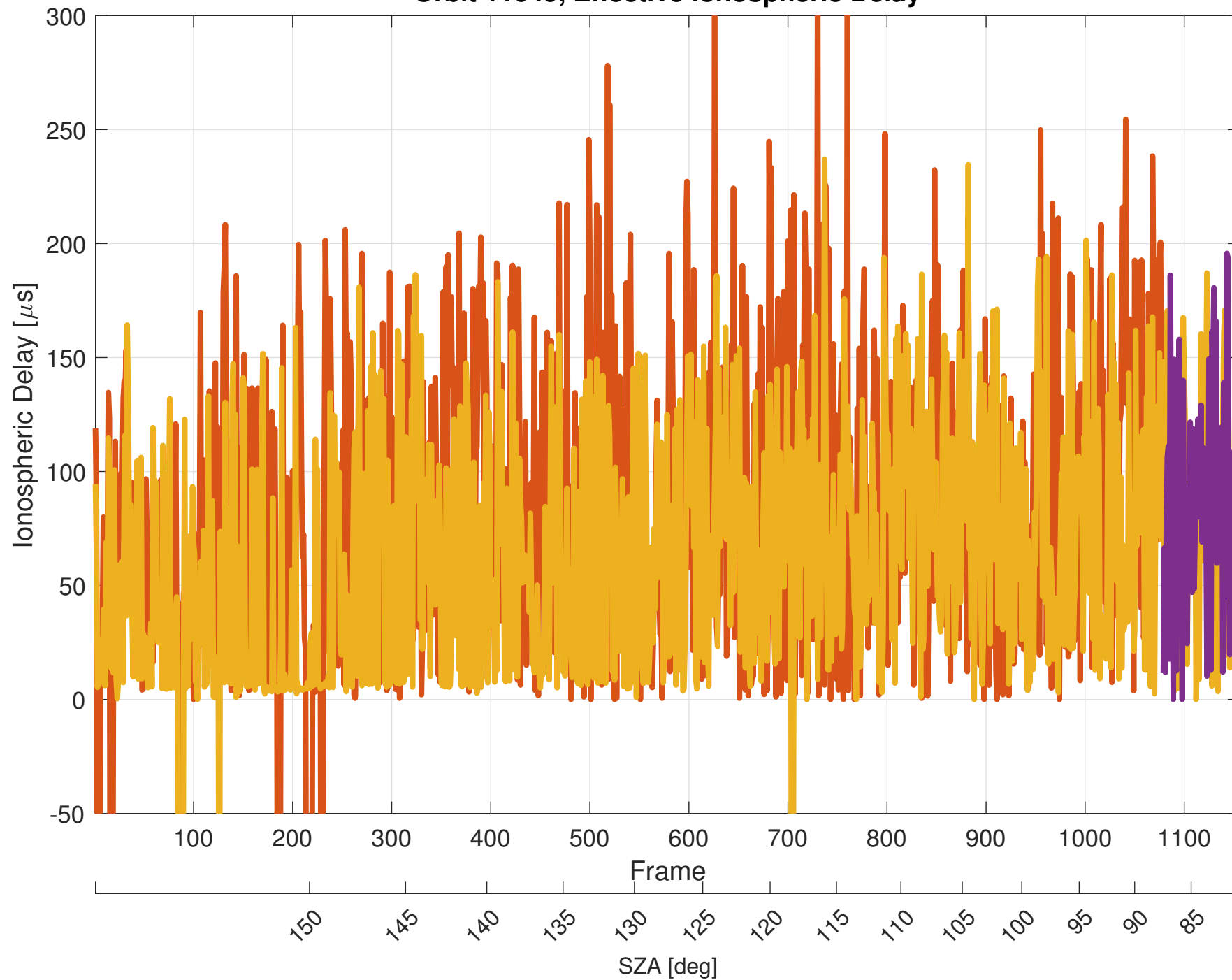
Orbit 11049, Effective Ionospheric Delay
