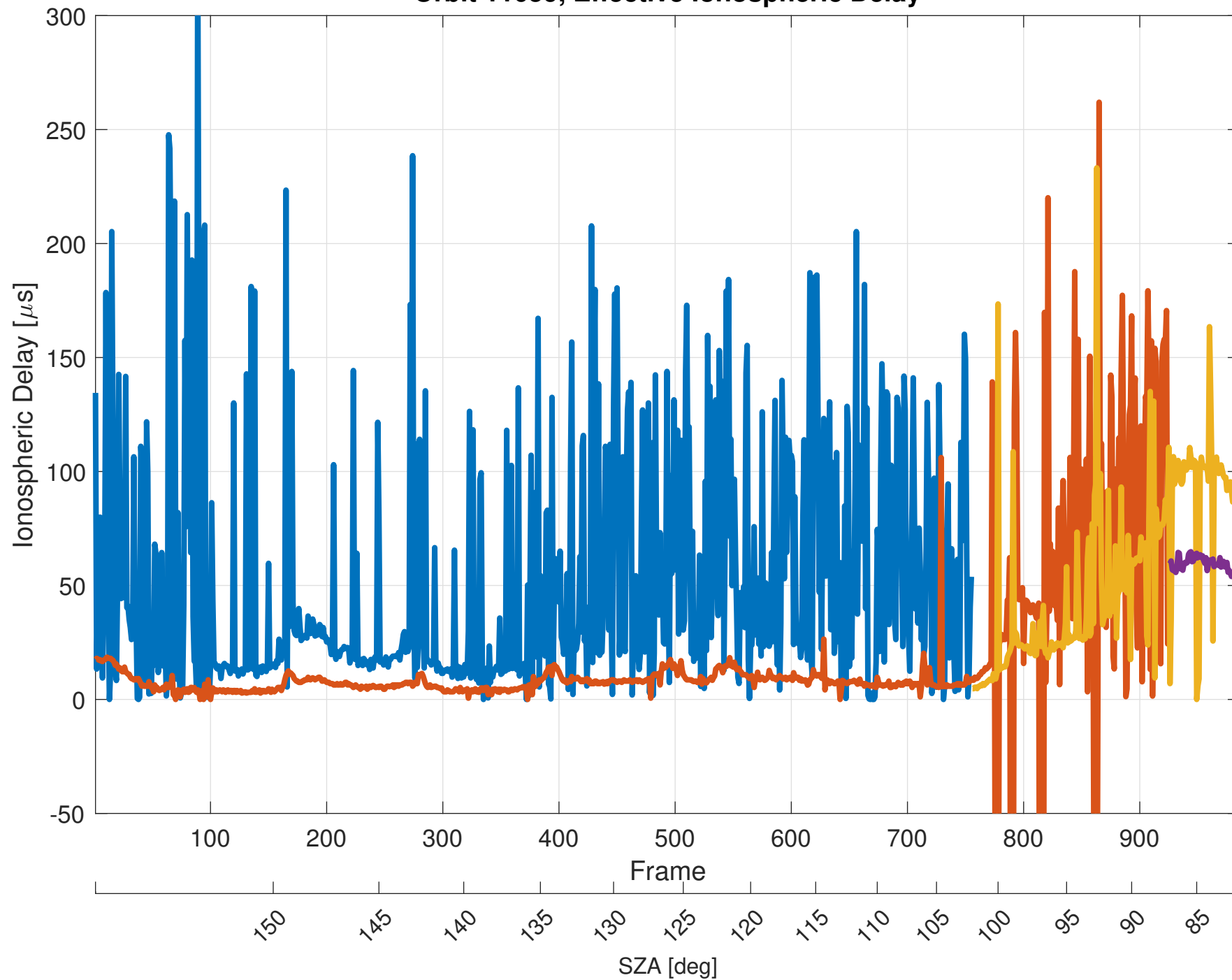
Orbit 11059, Effective Ionospheric Delay
