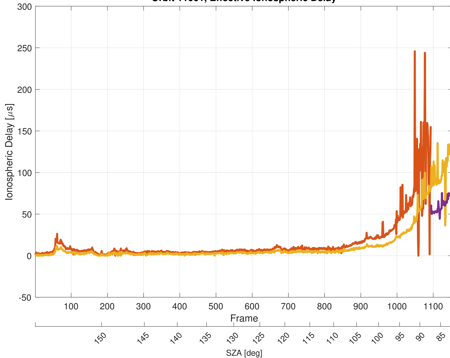
Orbit 11061, Effective Ionospheric Delay
