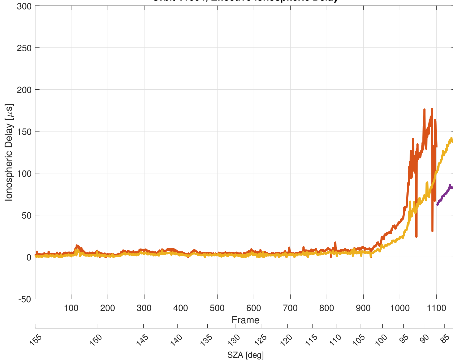
Orbit 11064, Effective Ionospheric Delay
