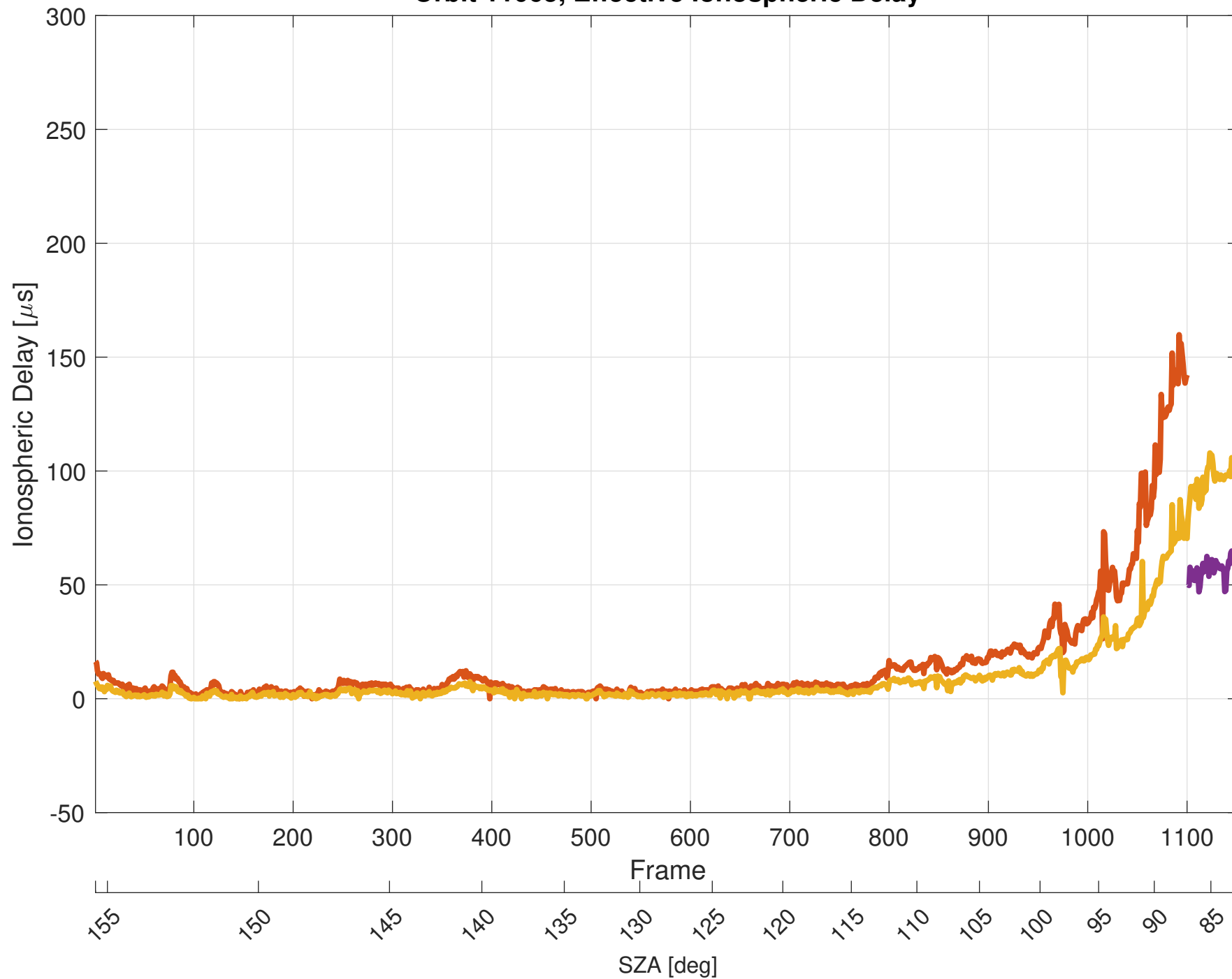
Orbit 11065, Effective Ionospheric Delay
