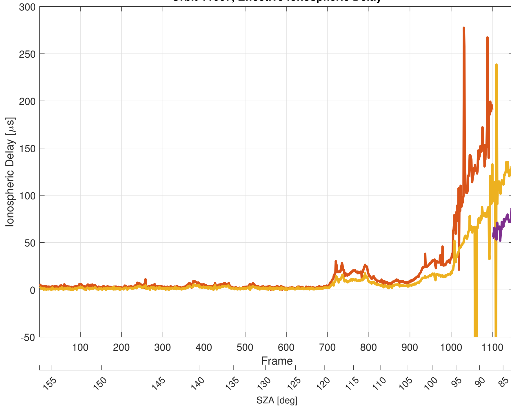
Orbit 11067, Effective Ionospheric Delay
