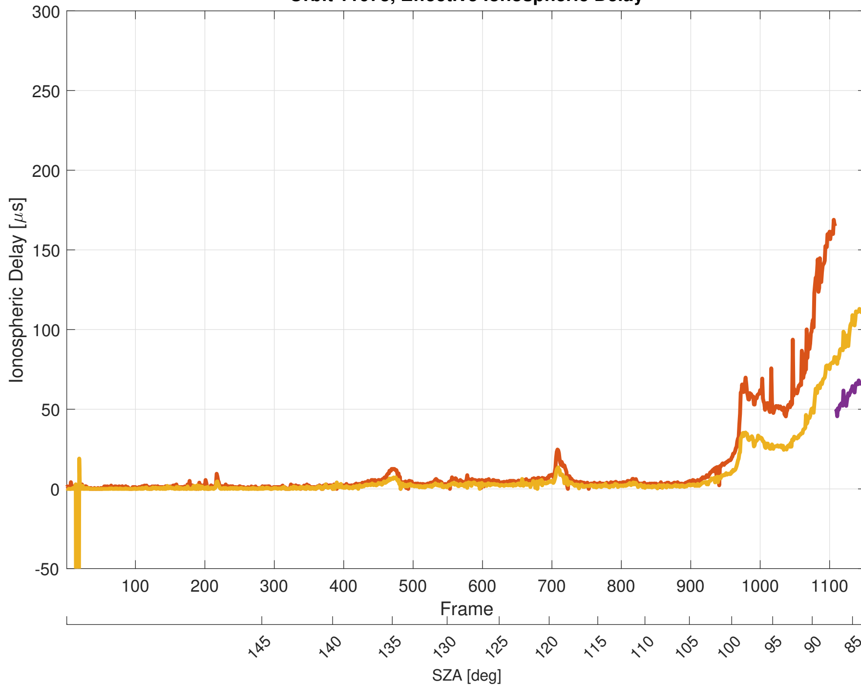
Orbit 11073, Effective Ionospheric Delay
