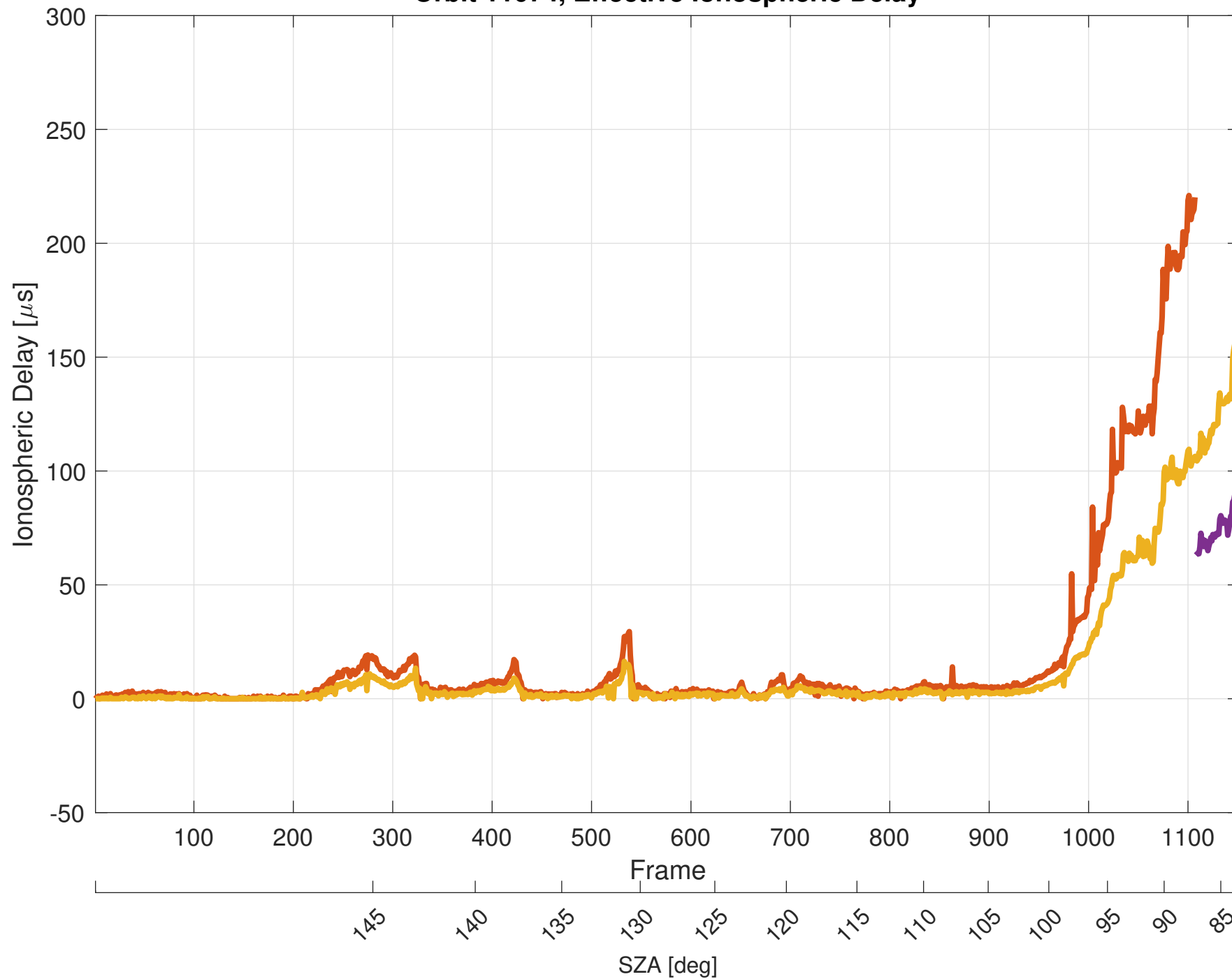
Orbit 11074, Effective Ionospheric Delay
