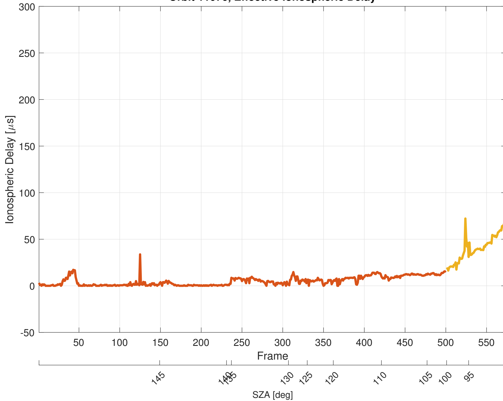
Orbit 11076, Effective Ionospheric Delay
