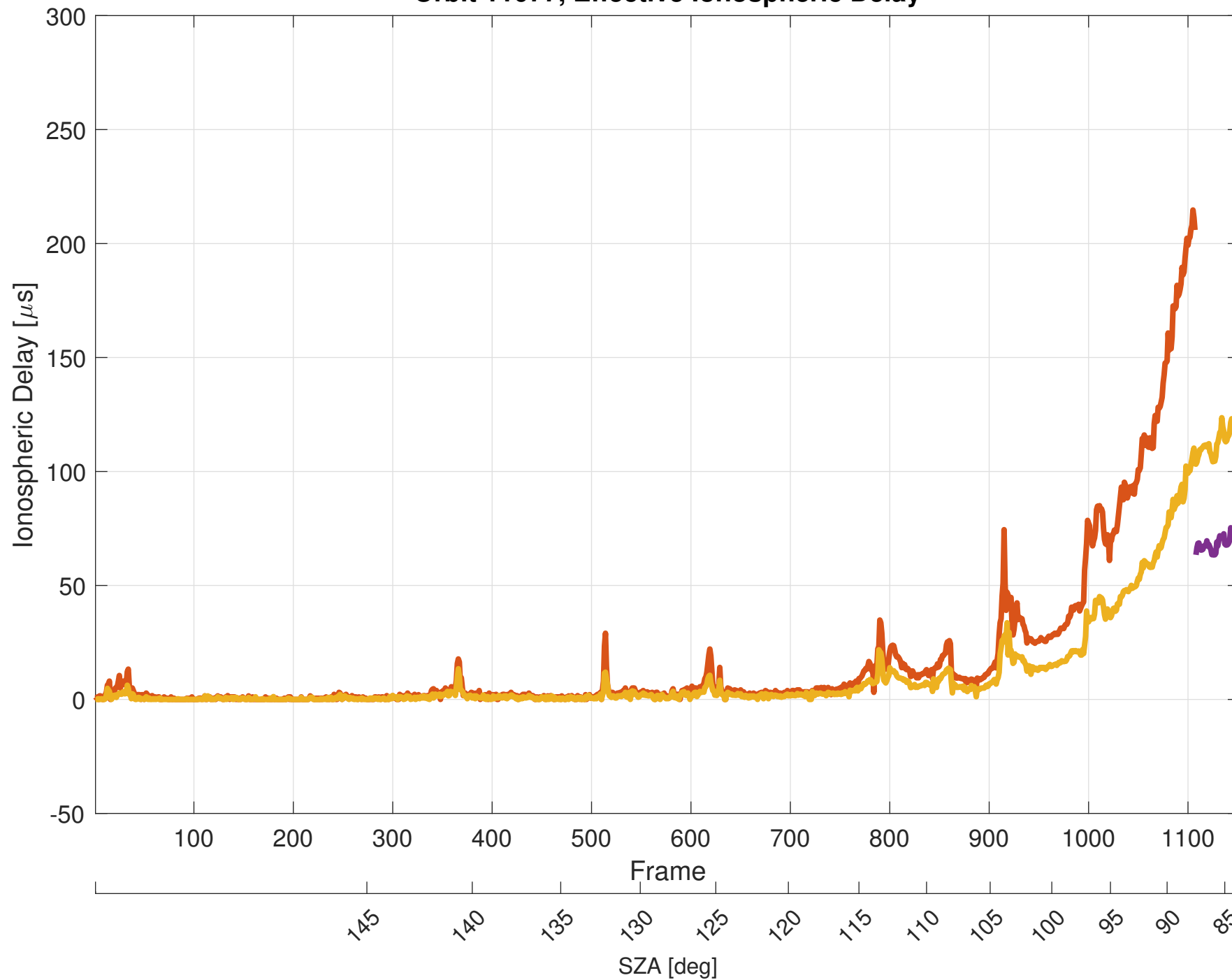
Orbit 11077, Effective Ionospheric Delay
