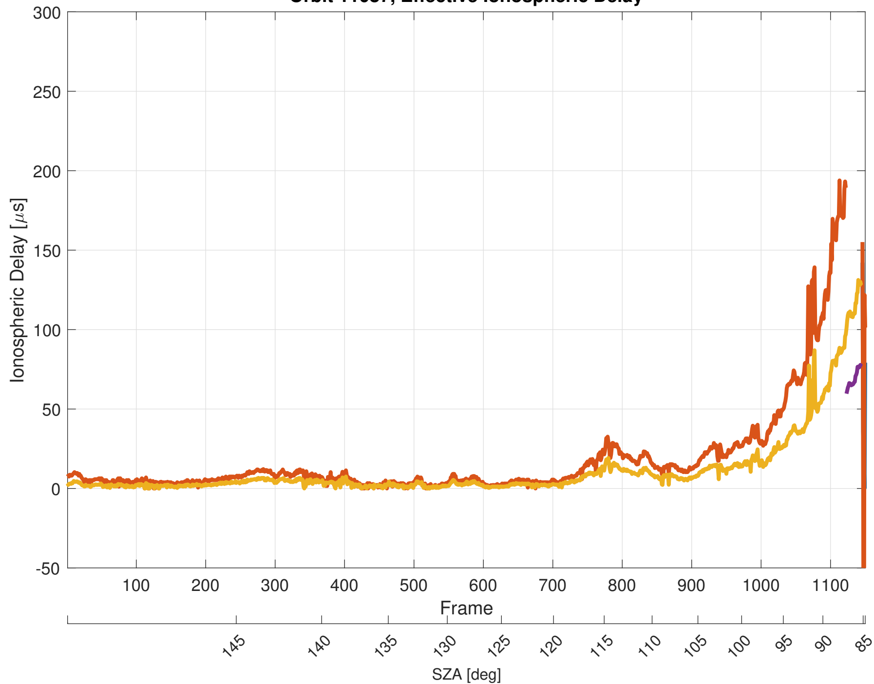
Orbit 11087, Effective Ionospheric Delay
