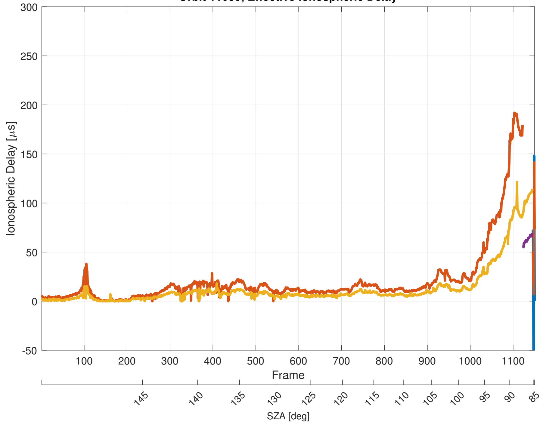
Orbit 11089, Effective Ionospheric Delay
